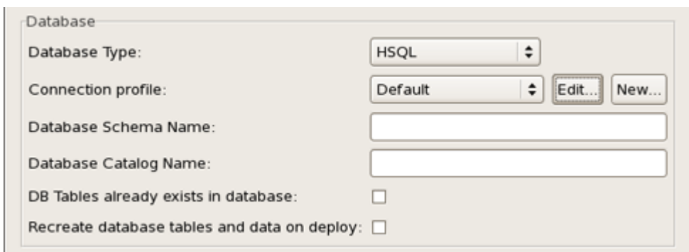
Figure 3.9. DataBase Setting
