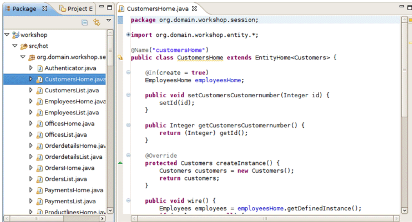
Figure 3.36. org.domain.workshop.entity Classes
