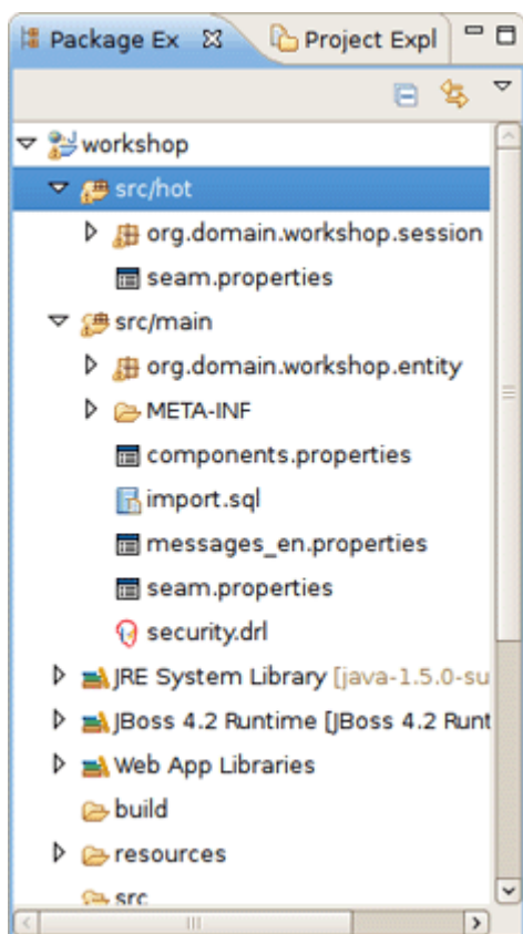
Figure 3.17. Project Structure
