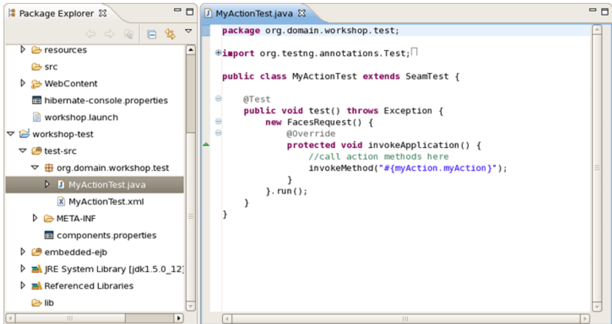
Figure 3.20. "workshop-test" Project
