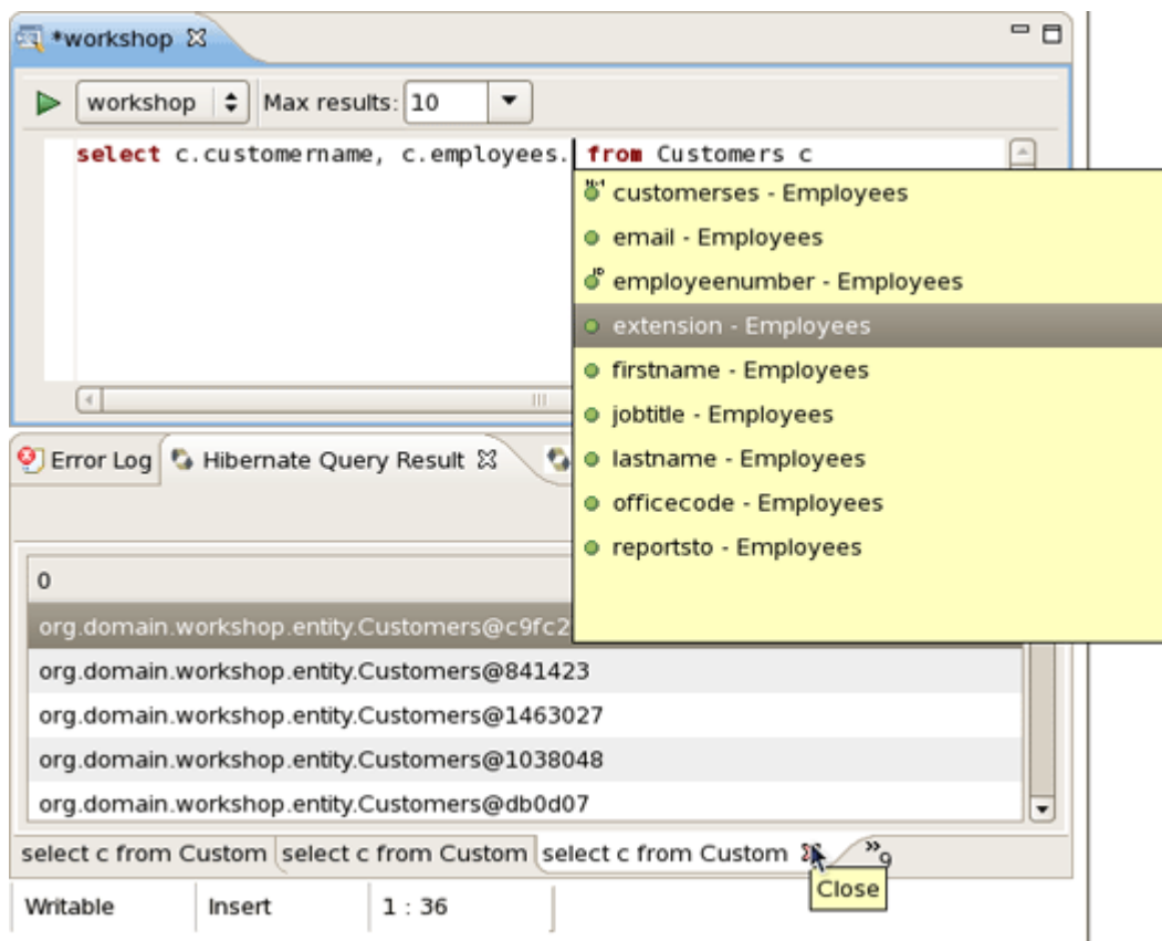
Figure 3.42. Code Completion
