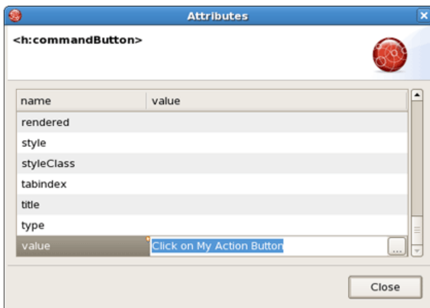
Figure 3.26. Attributes Dialog
