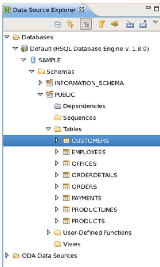
Figure 3.32. "CUSTOMERS" Table
