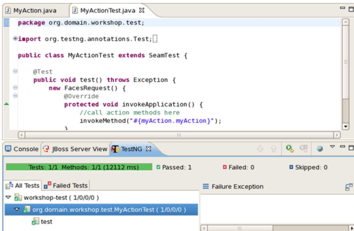
Figure 3.22. TestNG Results
