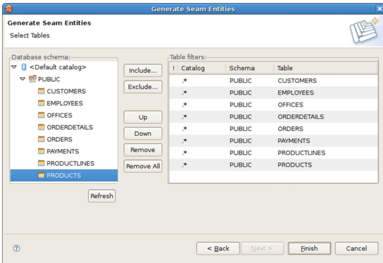
Figure 3.35. Selecting Tables
