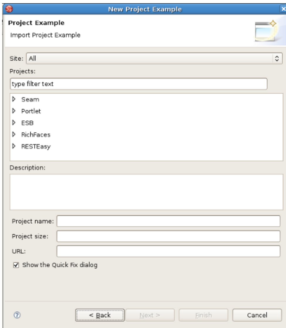
Figure 6.1. Project Examples
