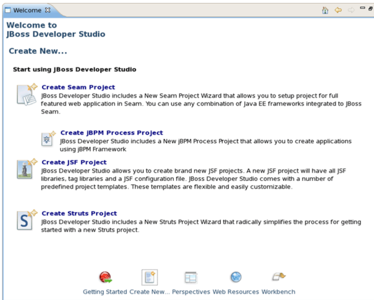
Figure 1.12. Create New...
