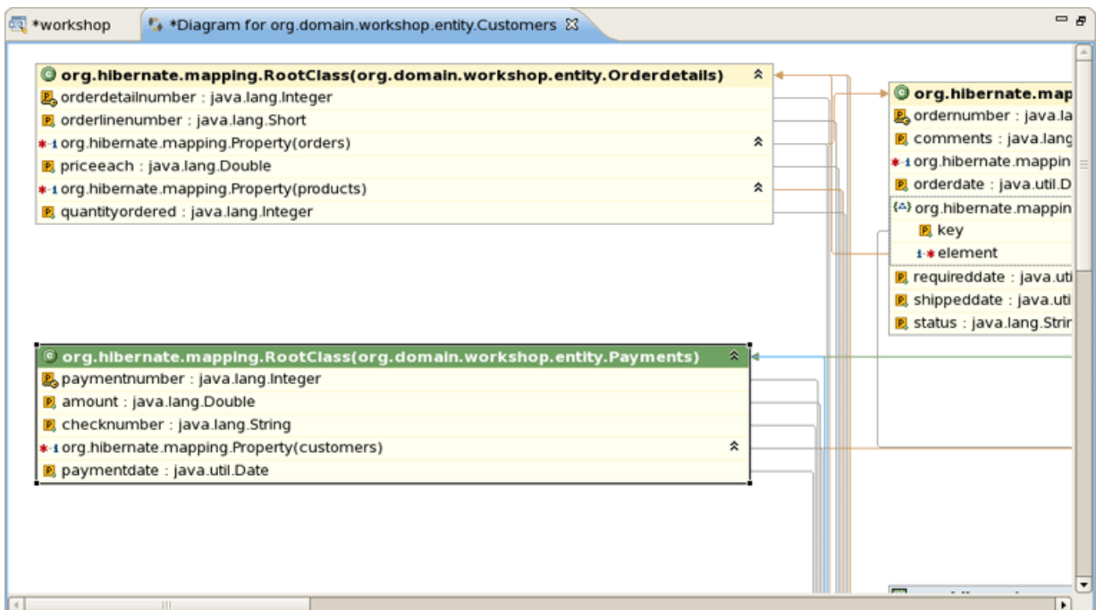
Figure 3.46. Diagram Tab
