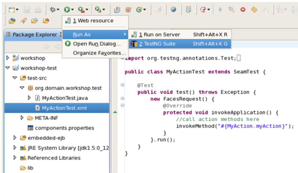
Figure 3.21. TestNG Running
