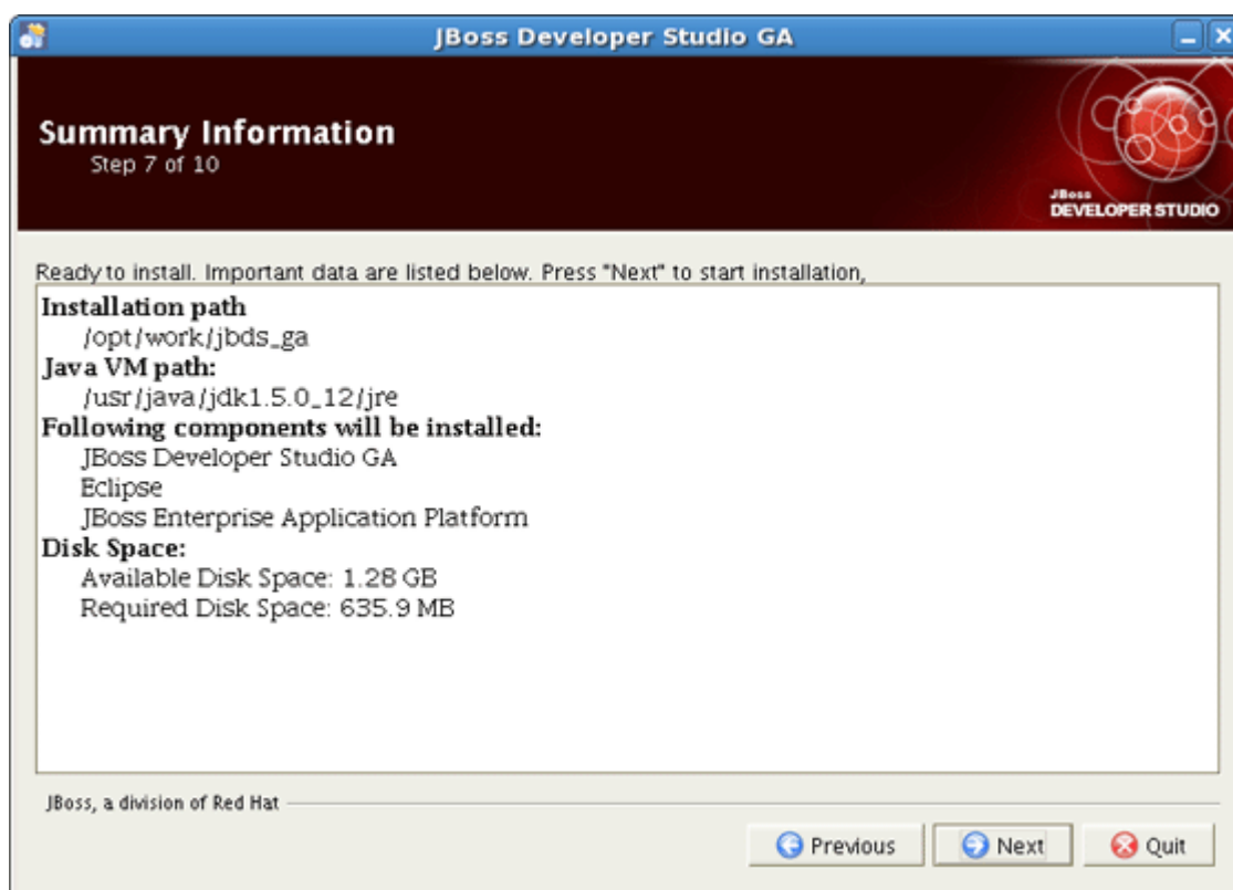
Figure 1.9. Summary Information
