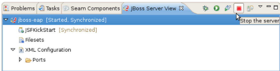
Figure 2.4. Stopping Server
