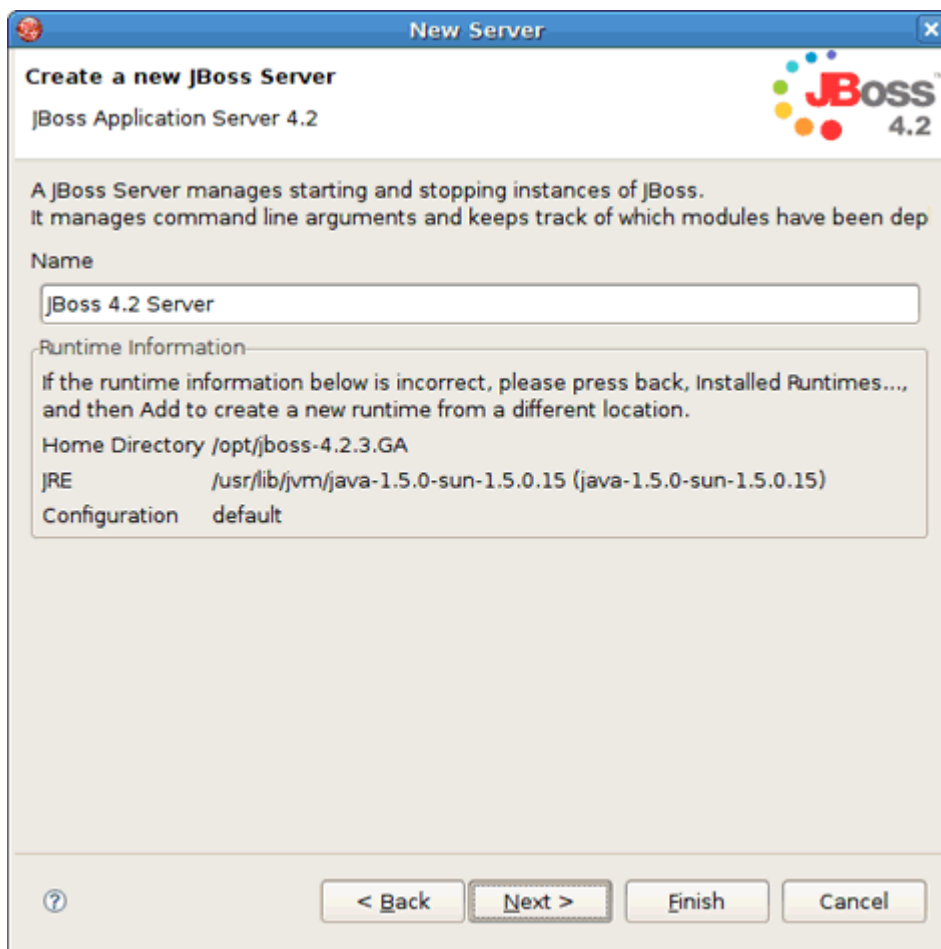
Figure 2.8. Configuring Projects
