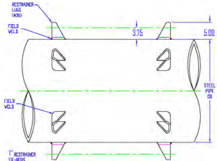
JCM 607 Restrainer Anchor Loops 1" Tie Rods
