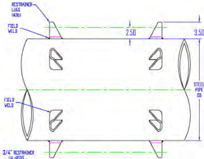
JCM 607 Restrainer Anchor Loops 3/4" Tie Rods
