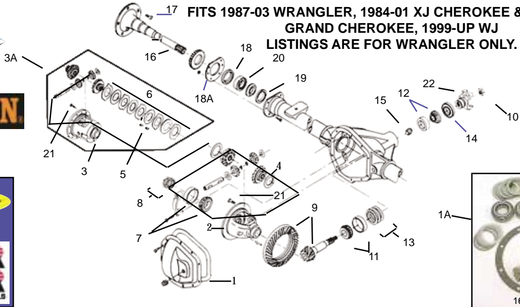
REAR DANA-35:
