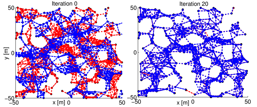
Fig. 2: Initial and final (after 20 steps) node locations (red) estimated by the distributed localization algorithm on a randomly generated graph with 300 nodes (blue) and 1288 edges (blue dotted lines)
