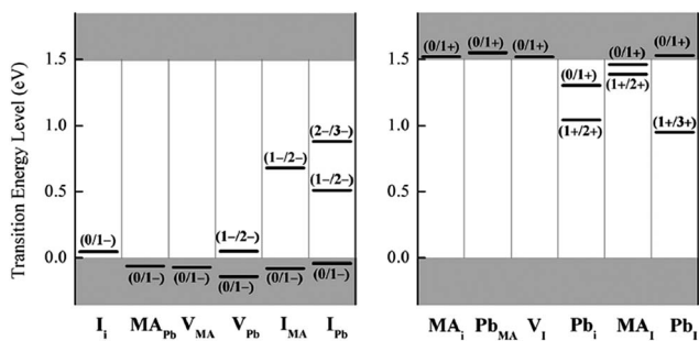
Fig. 7 Defect diagram of MAPbI _3 perovskite from DFT calculation: (Left) the intrinsic acceptors and (Right) intrinsic donors. Adapted with permission from ref. 80. 2014 American Institution of Physics.
