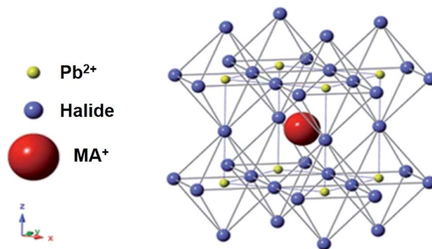
Fig. 1 Crystal lattice of the methylammonium lead halide ( \text{CH}_3\text{NH}_3\text{-PbX}_3 ) perovskite structure. Adapted with permission from ref. (7). Copyright 2013 Nature Publishing Group.
