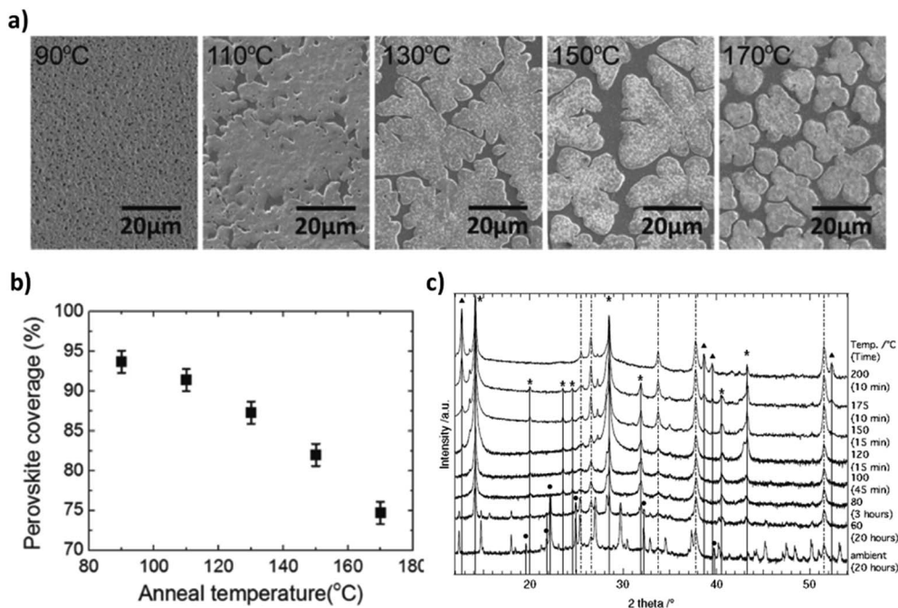
Fig. 10 One-step solution processed perovskite films annealed under different temperatures: (a) the top view SEM images; (b) the surface coverage; (c) the XRD spectra of perovskite films obtained under different annealing temperatures and time. Adapted with permission from ref. (65 and 96). Copyright 2013 Wiley.
