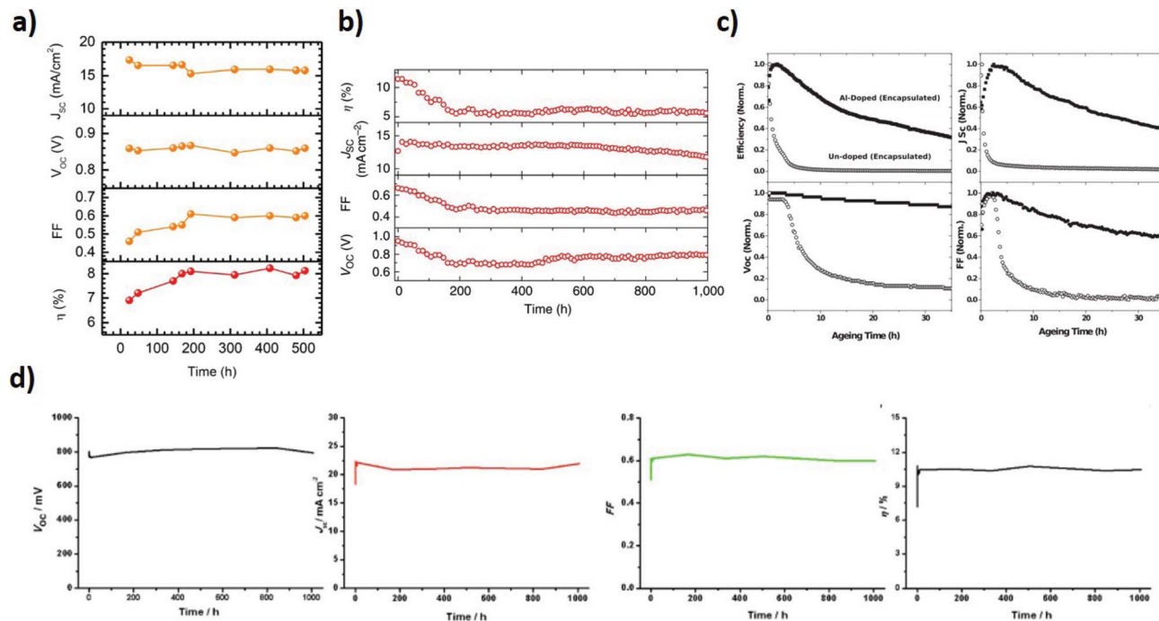
Fig. 16 Long term stability tests of perovskite devices and the photovoltaic parameters: (a) all solid state MAPbI 3 perovskite devices without encapsulation under white light illumination for over 500 h in air; (b) replacing TiO 2 with Al 2 O 3 to prevent the photochemical reaction by UV light, the encapsulated device stabilized after 200 h under 40 °C with full spectrum illumination; (c) Al doped TiO 2 was used to reduce the surface defects of TiO 2 , the encapsulated devices were performed to show an improved stability. (d) HTL free, (5-AVA) x (MA) 1-x PbI 3 perovskite device based on ZrO 2 as the mesoporous scaffold and carbon as the electrode demonstrated more than 1008 h stability under full sunlight illumination without encapsulation. Adapted with permission from ref. (77, 87, 114 and 116). Copyright 2014 Nature Publishing Group, 2014 American Association for the Advancement of Science.
