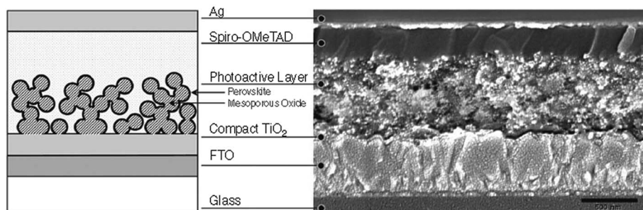
Fig. 4 (Left) The schematic diagram and (Right) cross-section SEM of the mesoporous structured perovskite solar cell device. Adapted with permission from ref. (50). Copyright 2013 American Association for the Advancement of Science.
