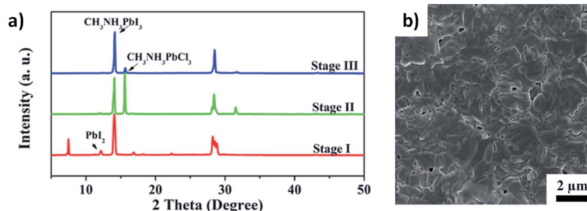
Fig. 12 (a) The XRD spectra of perovskite films annealed under 90–105 °C for different time; (b) the top view SEM images of the perovskite film annealed for 85 min under mild moisture conditions. Adapted with permission from ref. (35). Copyright 2014 American Association for the Advancement of Science.
