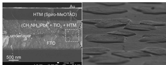
Fig. 13 (Left) Cross-section and (Right) surface SEM images of the MAPbI 3 -coated mp-TiO 2 film. Adapted with permission from ref. (53 and 87). Copyright 2013 Nature Publishing Group.
