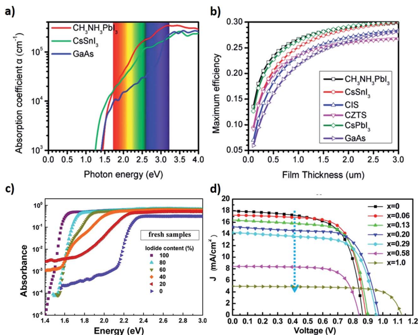
Fig. 8 (a) The calculated absorption coefficient of \text{MAPbI}_3 , \text{CsSnI}_3 and \text{GaAs} materials, respectively. (b) The calculated maximum PCE of different photovoltaic absorber materials at different film thicknesses. (c) Absorbance spectra of different ratios of Br in \text{MAPbI}_{3-x}\text{Br}_x materials. (d) J - V curves of different Br ratios in \text{MAPbI}_{3-x}\text{Br}_x devices. Adapted with permission from ref. (20, 73 and 84). Copyright 2014 Wiley, 2014 American Chemical Society.
