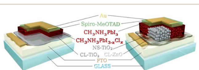
Fig. 2 Perovskite solar cell device structure: (Left) planar structure, (Right) mesoporous scaffold. Adapted with permission from ref. (39). Copyright 2014 American Chemical Society.
