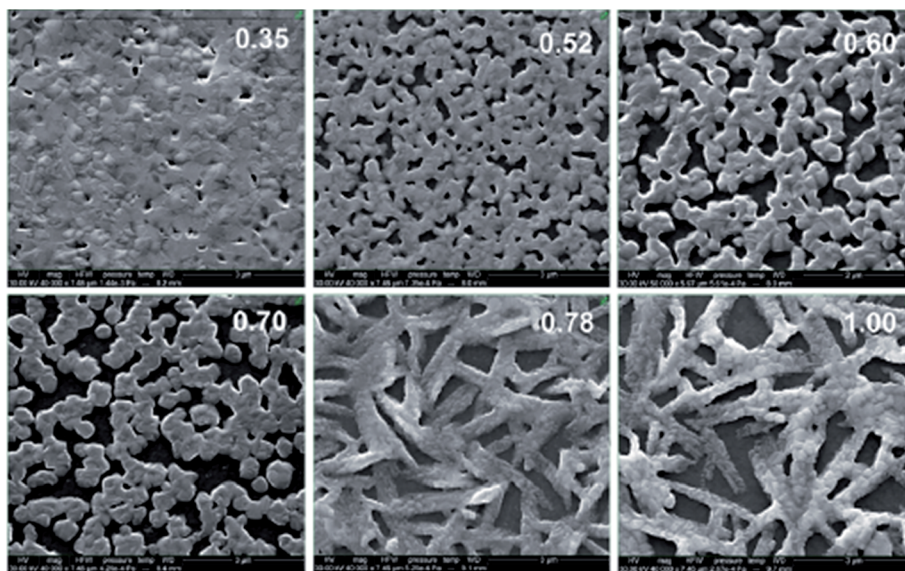
Fig. 9 The top view SEM images of the perovskite films prepared from different mole ratios of \text{PbI}_2 to MAI dissolved in DMF. Adapted with permission from ref. (34). Copyright 2014 The Royal Society of Chemistry.
