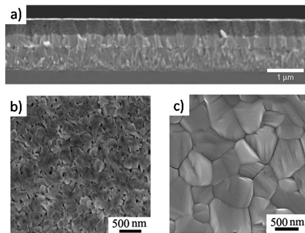
Fig. 5 (a) Cross-section SEM images of the perovskite film prepared by dual source coevaporation. The perovskite layer with homogeneous and flat boundaries can be distinguished clearly. (b) The as-deposited \text{PbI}_2 layer by solution process and (c) the perovskite film with micrometer grain size, obtained by the vapor assisted solution process. Adapted with permission from ref. (32 and 33). Copyright 2013 Nature Publishing Group, 2014 American Chemical Society.
