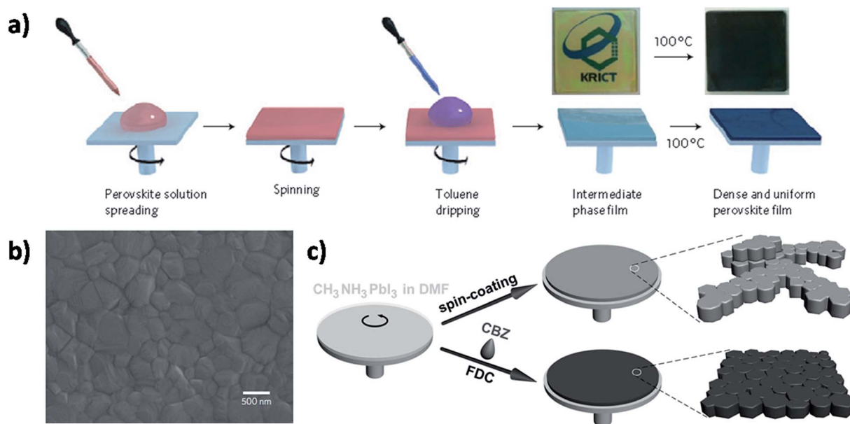
Fig. 14 (a) Schematic illustration of perovskite films prepared from DMSO/GBL mixed solvent and dripped with toluene and (b) the top view SEM of the perovskite film from this method. (c) Schematic illustration of the perovskite film deposited and immediately treated with chlorobenzene. Adapted with permission from ref. (54 and 107). Copyright 2014 Nature Publishing Group, 2014 Wiley.
