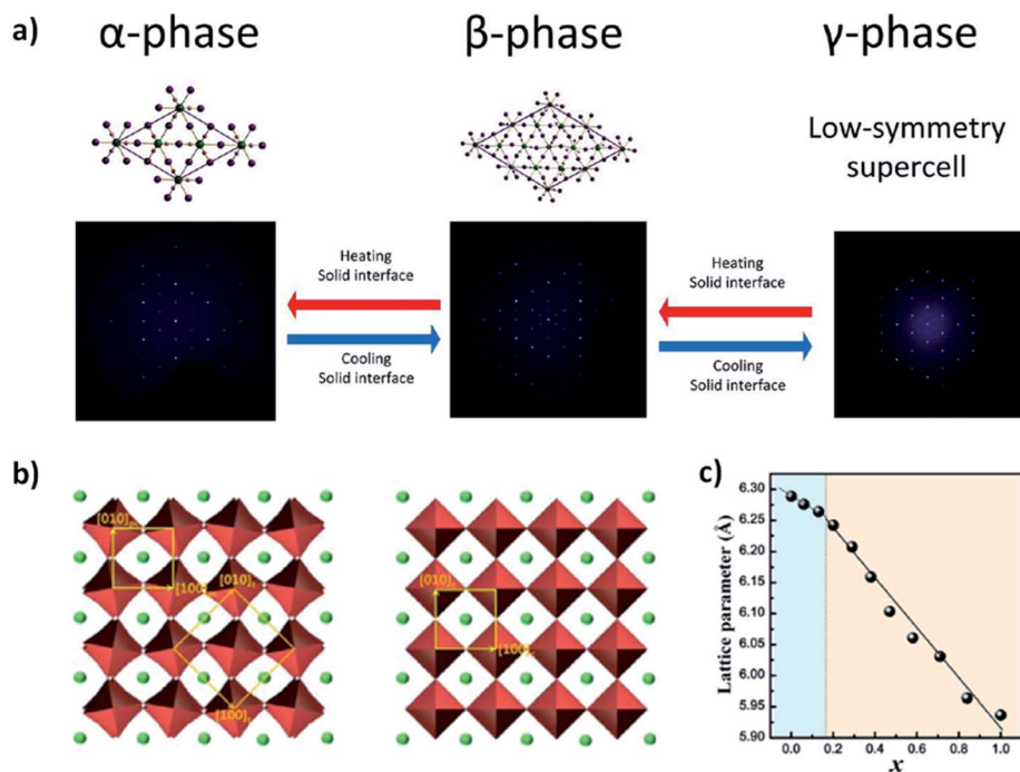
Fig. 6 (a) Graphical scheme of observed phase transitions of MA(Pb,Sn) X_3 perovskite materials. Precession images are drawn at [006] view. (b) The structure transformation from the Br incorporation in MAPbI _3 and (c) the lattice contact change with different amounts of Br incorporation. Adapted with permission from ref. (68 and 73). Copyright 2014 American Chemical Society.
