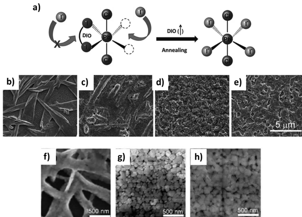
Fig. 11 (a) The proposed mechanism of DIO interaction with the \text{PbX}_2 complex. The top view SEM images: (b–e) perovskite films from different amounts of MACl treatment; (f–g) perovskite films from different amounts of \text{NH}_4\text{Cl} treatment. Adapted with permission from ref. (100–102). Copyright 2014 Wiley, 2014 American Chemical Society, 2014 The Royal Society of Chemistry.
