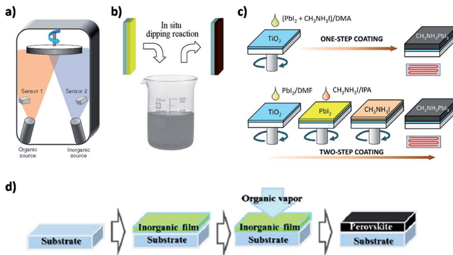
Fig. 3 The preparation of MAPbI 3-x Cl x film from different deposition methods: (a) Dual source coevaporation using PbCl 2 and MAI source. (b) Sequential deposition by dipping the PbI 2 film into MAI solution. (c) One-step solution process based on the mixture of PbI 2 and MAI, and sequential coating of PbI 2 and MAI. (d) Vapor-assisted solution process using the MAI organic vapor to react with the PbI 2 film. Adapted with permission from ref. (32, 33, 44 and 45). Copyright 2013 Nature Publishing Group, 2014 American Institution of Physics, 2014 American Chemical Society.
