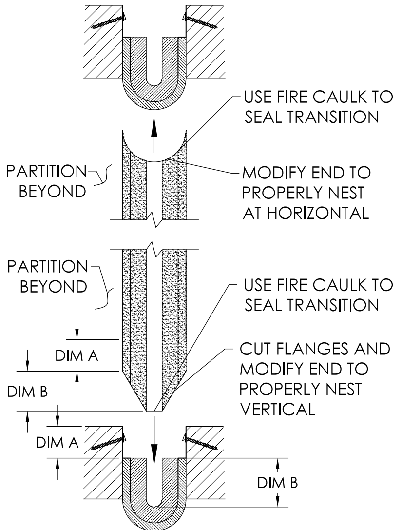
Fig 3 TRANSITION INTERSECTION DETAIL
