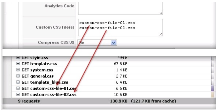
Custom CSS files are loaded with other template CSS files
