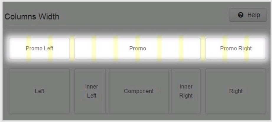
12 Bootstrap grids
