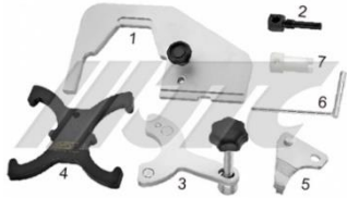
JTC-4153 VOLVO TIMING TOOLS SET (T4, T5)
