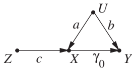
Figure 10 Bias amplification, \beta_{yx \cdot z} - \gamma_0 > ab , produced by conditioning on an instrumental variable ( Z ).
