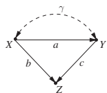
Figure 6 Conditioning on Z = 1 represents inclusion in the dataset and biases the regression of Y on X , unless c = 0 .
