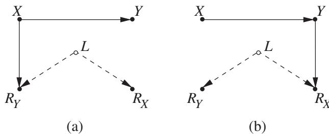
Figure 7 Missingness diagrams in which conditioning on R_x = 0 or R_y = 0 represents unmasking the values of X and Y , respectively. The parameter \sigma_{xy} , \sigma_x^2 and \sigma_y^2 can all be estimated bias-free from data generated by either model, through each model requires a different estimation procedure.
