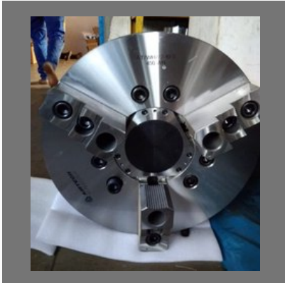
Airtech 450WH Open Centre Power Chuck
