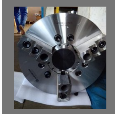
Airtech 250WH Open Centre Power Chuck
