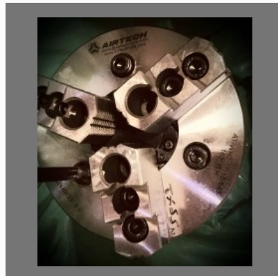
Airtech 165WH Open Centre Power Chuck
