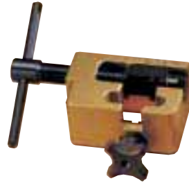
Sight Pusher Adjustment tool for P220, P225, P226, P228, P229, P239, P245 and sig pro models
