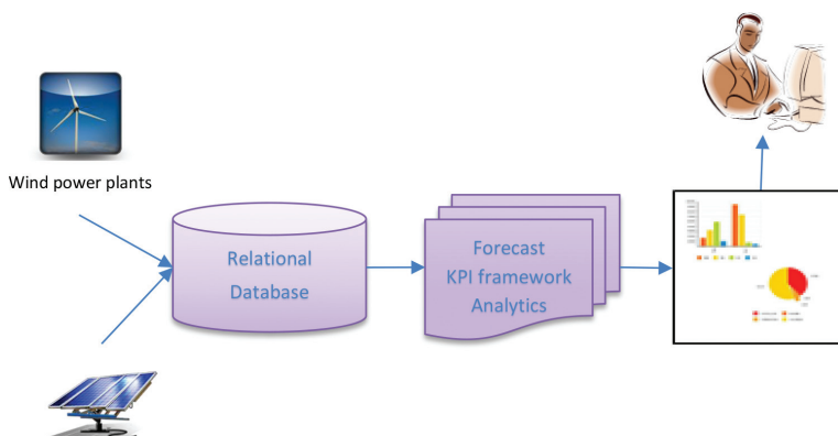
Figure 1. SIPAMER's architecture.
