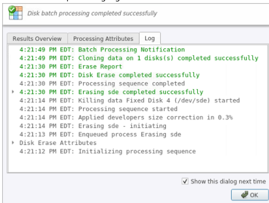
Figure 25: Log Sample
