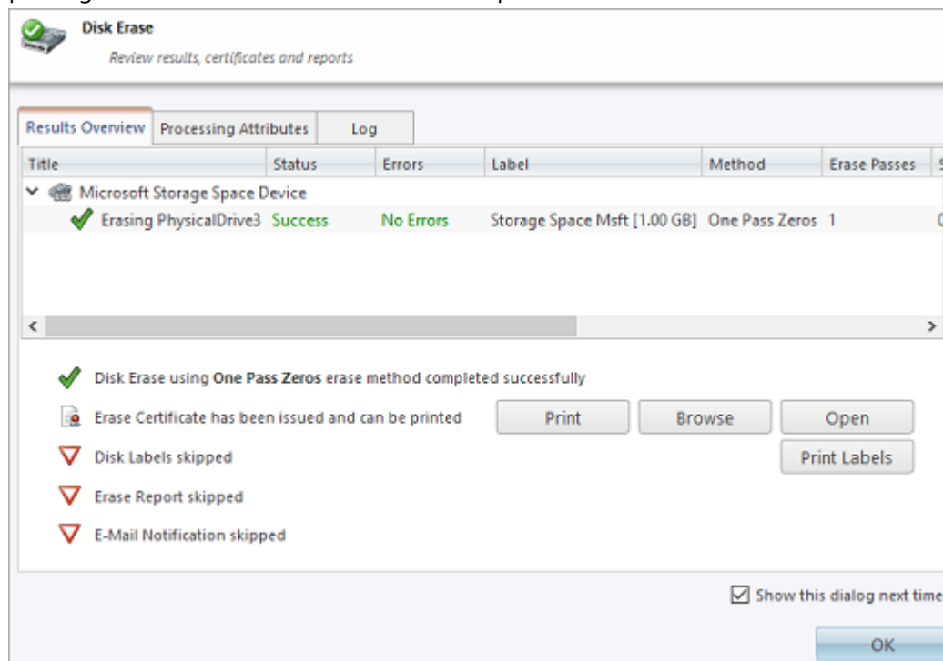
Figure 16: Erase Summary
