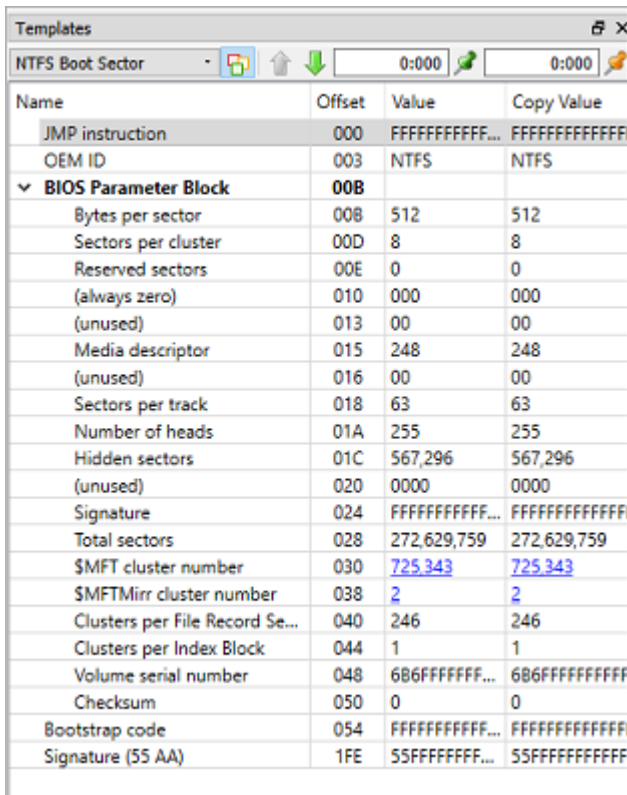
Figure 44: NTFS Boot Sector Template View
