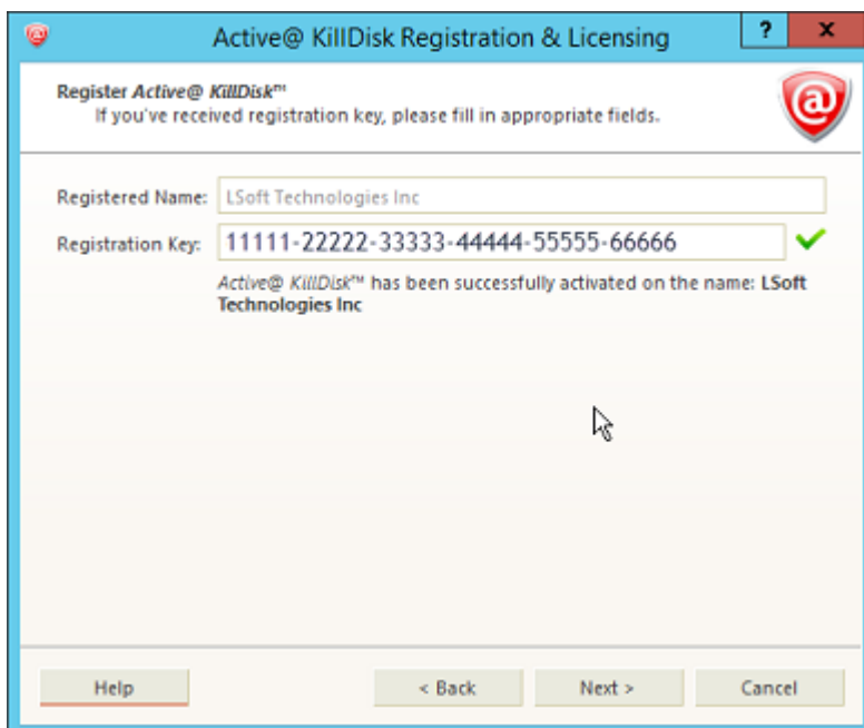
Figure 2: Registration Complete
