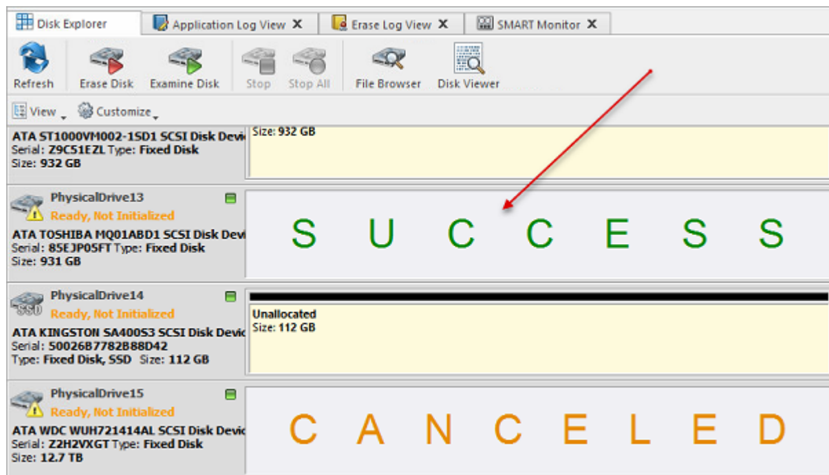
Figure 15: Erase Completed
