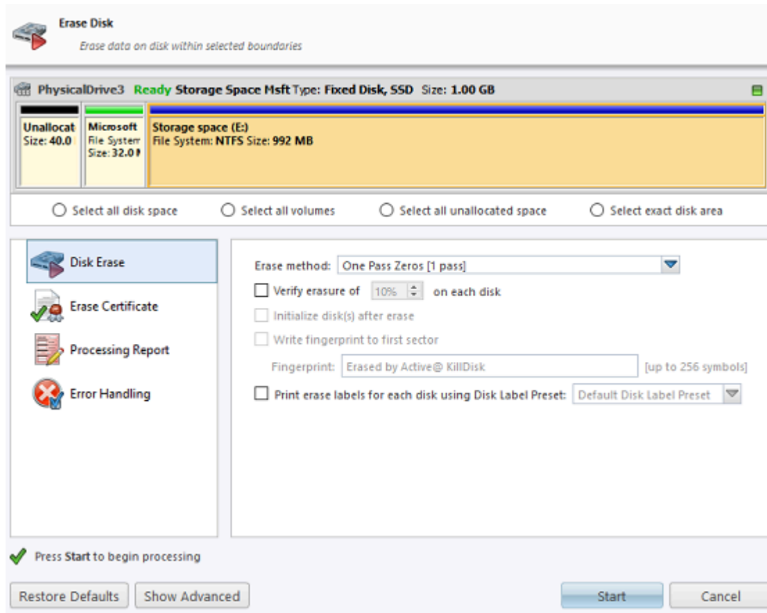
Figure 12: Erase Options
