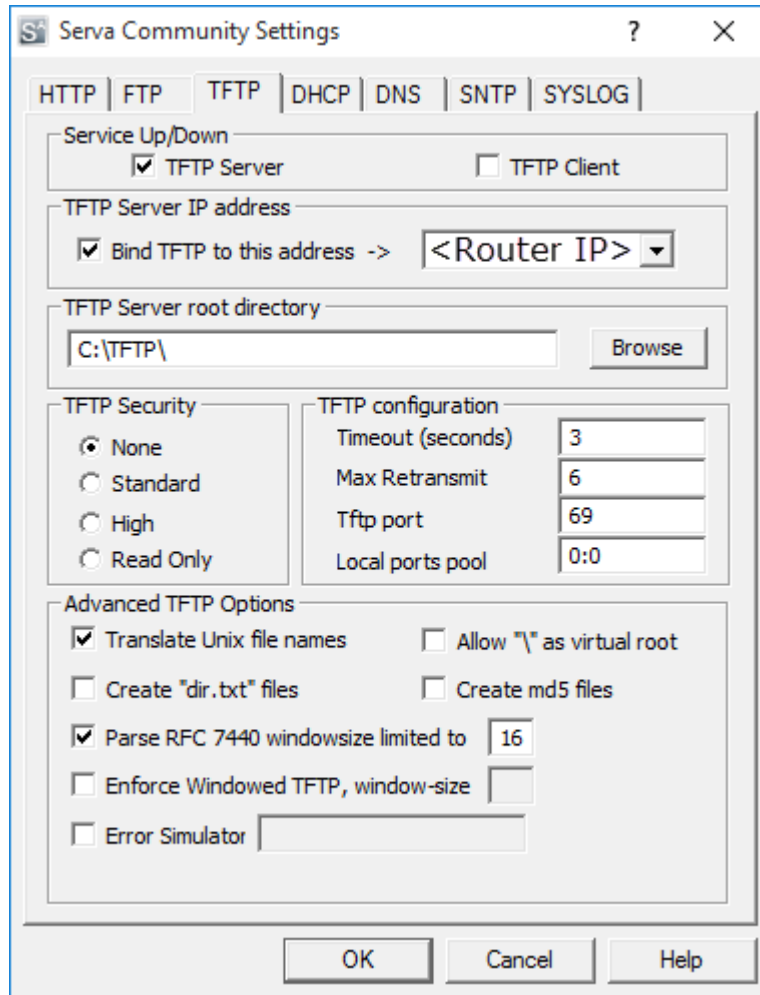
Figure 59: TFTP Configuration
