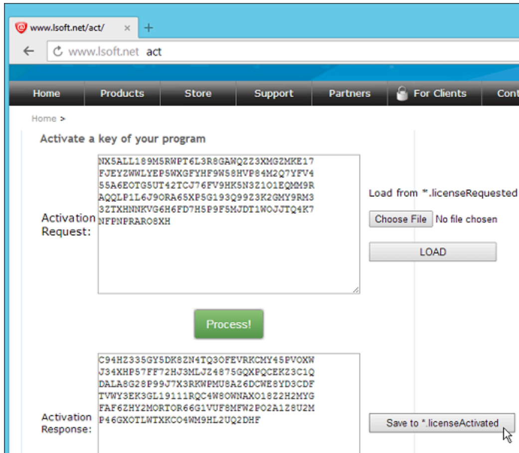
Figure 5: Activate in Browser
