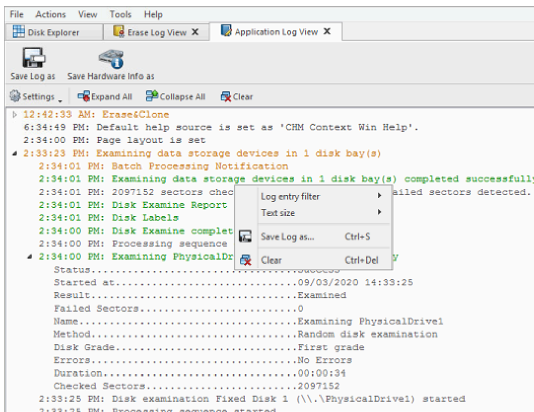
Figure 48: Application Log View
