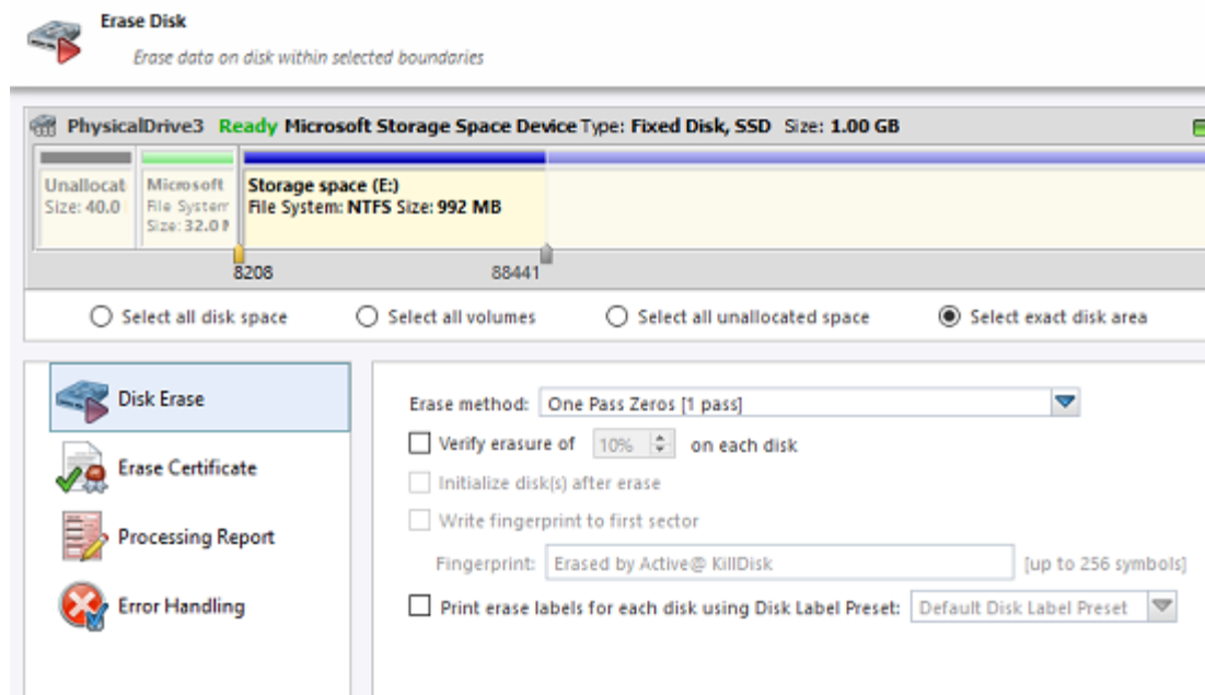
Figure 17: Erase a Specific Area
