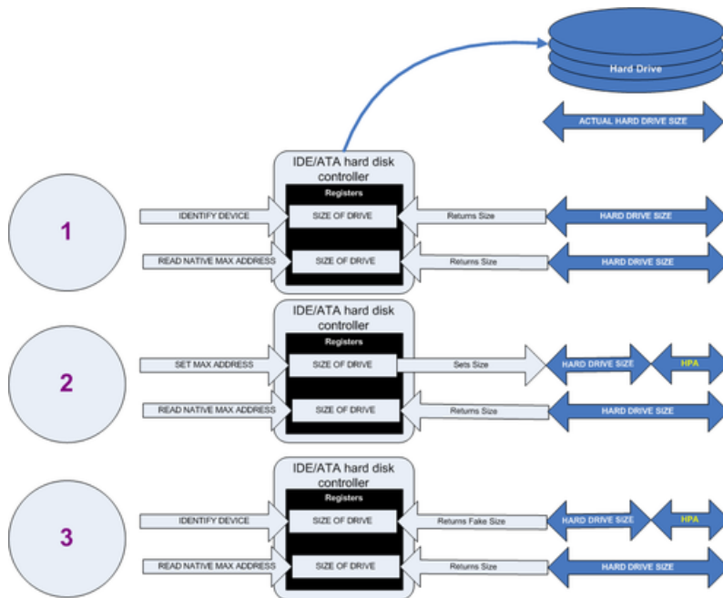
Figure 62: Creation of an HPA
