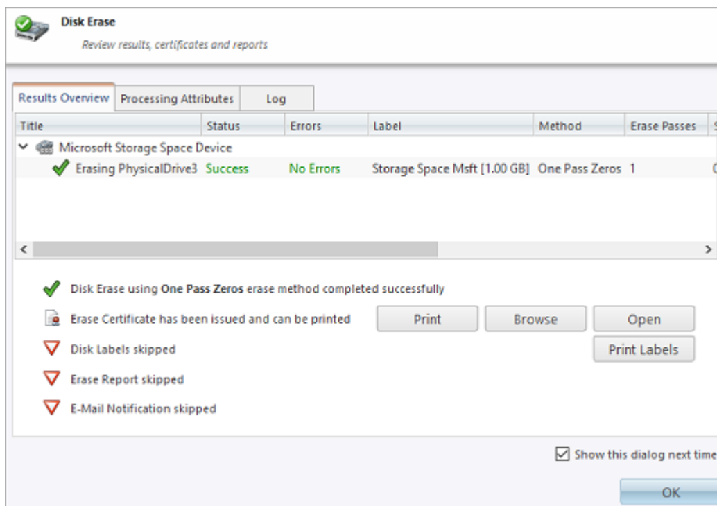
Figure 31: Print Labels from Processing Summary
