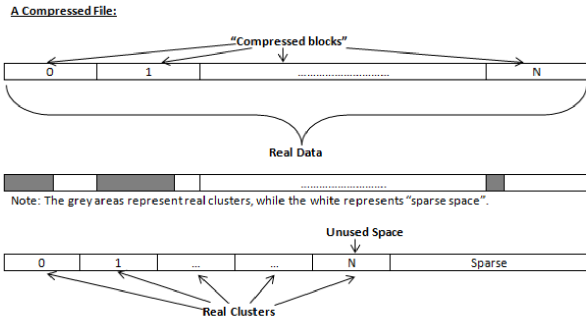
Figure 51: Compressed File Structure
