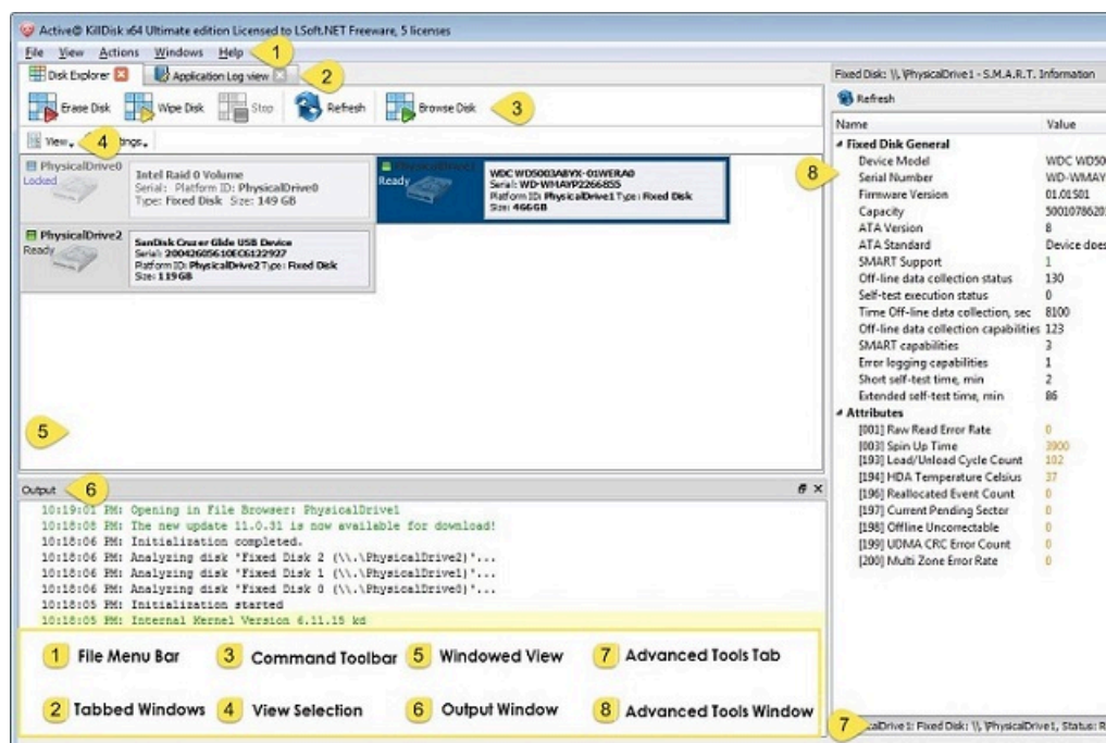
Figure 9: KillDisk Dashboard
