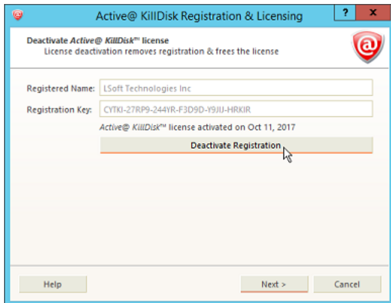
Figure 7: Deactivating Registration
