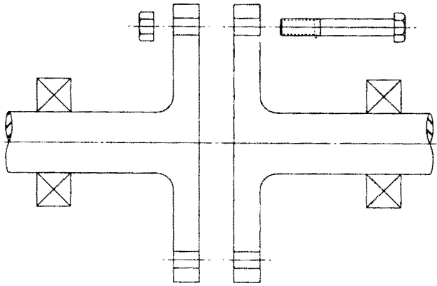
Figure 1. Rigid Couplings.
