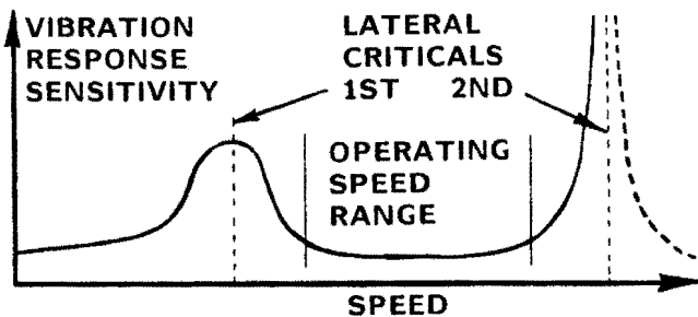
Figure 52. Super-Critical Vibration Response vs Operating Speed.
