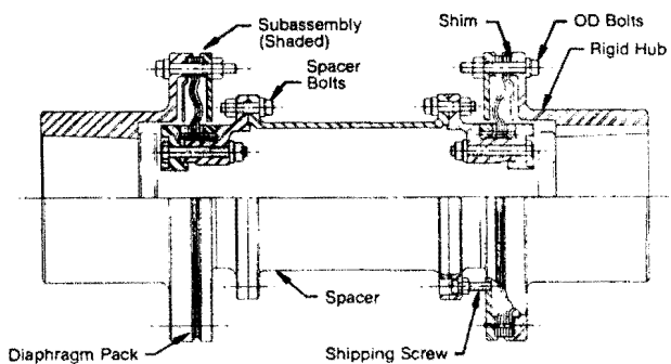
Figure 31. HP Series (high performance).
