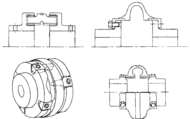
Figure 19. Types of Nonmetallic Couplings.
