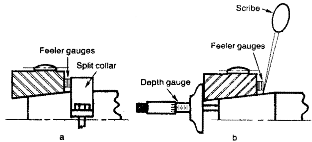
Figure 60. Means to Measure Hub Advance.
