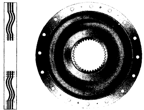
Figure 30. Multiple Convoluted Diaphragm Pack.
