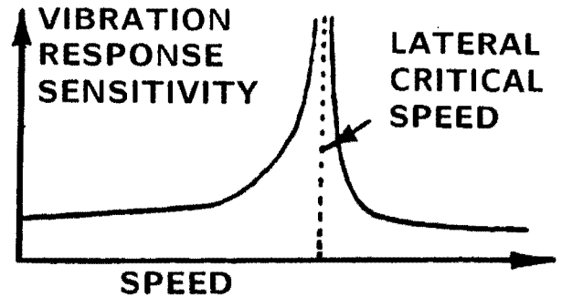
Figure 46. Subcritical Vibration Response vs. Operating Speed.
