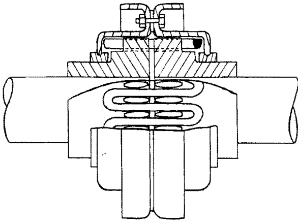
Figure 16. Grid Type Coupling.
