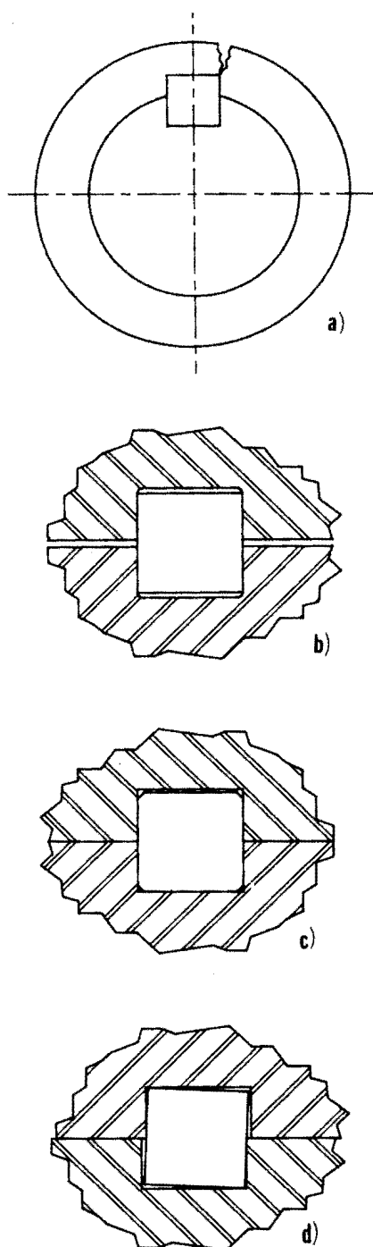
Figure 61. Problems with Key Misfits. a) tall key can crack hub; b) result of sharp keys no chamfers; c) keys must be chamfered; d) results of loose key.
