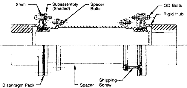
Figure 33. RR Series (reduced ratio).
