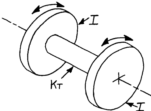
Figure 44. Machines' Inertia and Coupling Stiffness.
