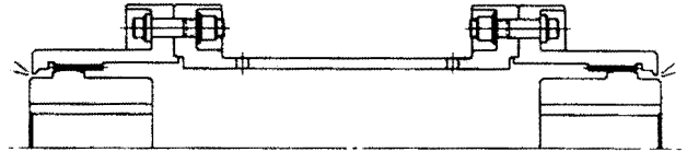
Figure 23. Reduced Moment Gear Coupling.
