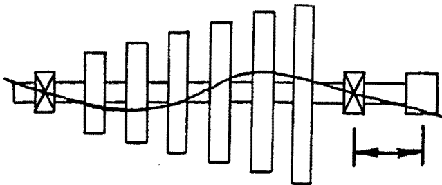
Figure 51. Machine With "Flexible Shaft."
