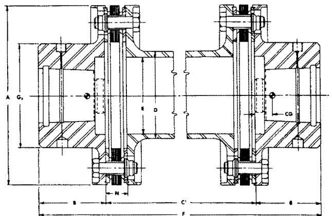
Figure 35. Marine Style Disc Couplings.
