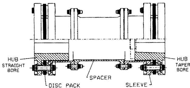
Figure 37. Reduced Moment Disc Coupling.
