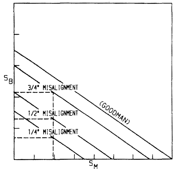
Figure 42. Goodman Diagram.
