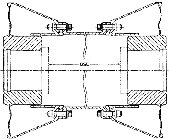
Figure 28. Reduced Moment Contoured Diaphragm Coupling.
