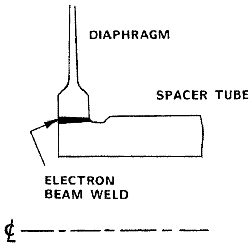
Figure 25. Contoured Diaphragm Welded to Spacer Tube.
