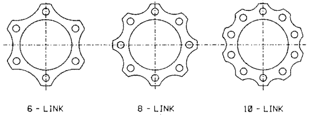
Figure 34. Disc/Link Shapes.
