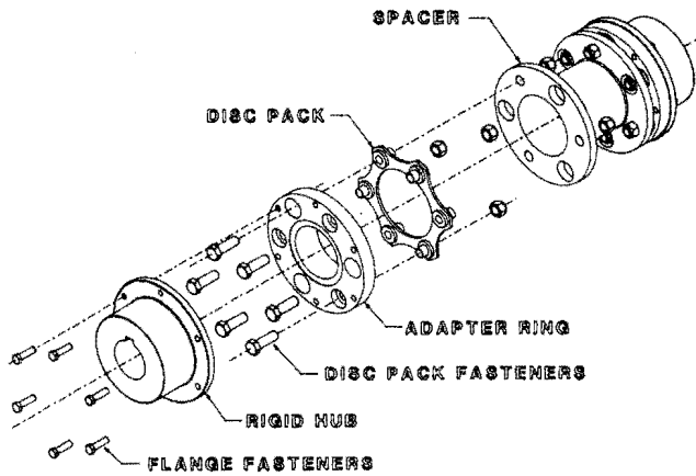
Figure 36. Marine Style Disc Couplings.
