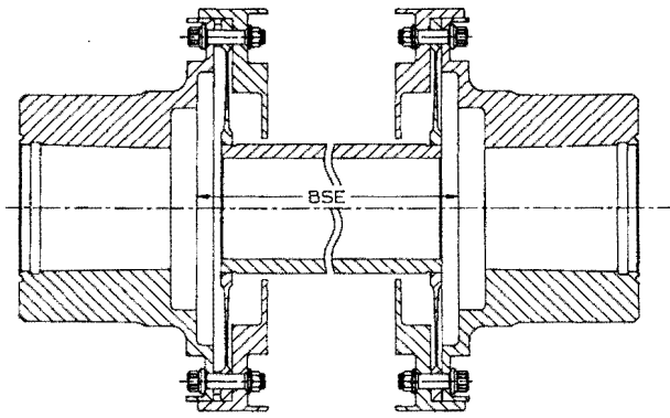
Figure 27. Piloted Contoured Diaphragm Coupling.
