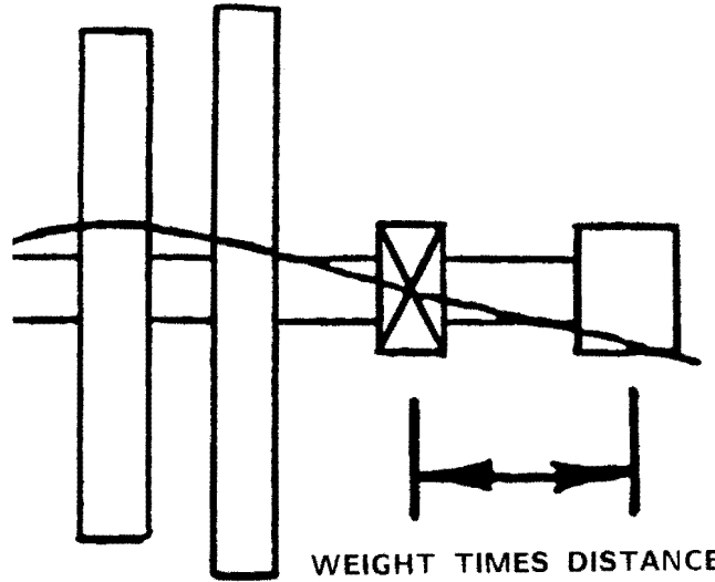
Figure 53. Coupling Weight to Node Point Distance.
