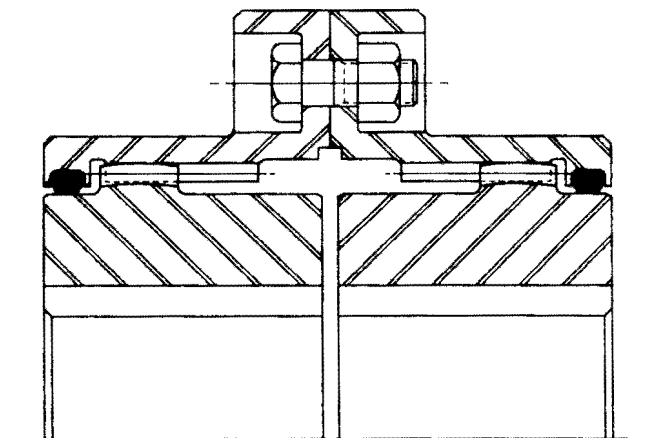
Figure 8. Typical Gear Coupling.
