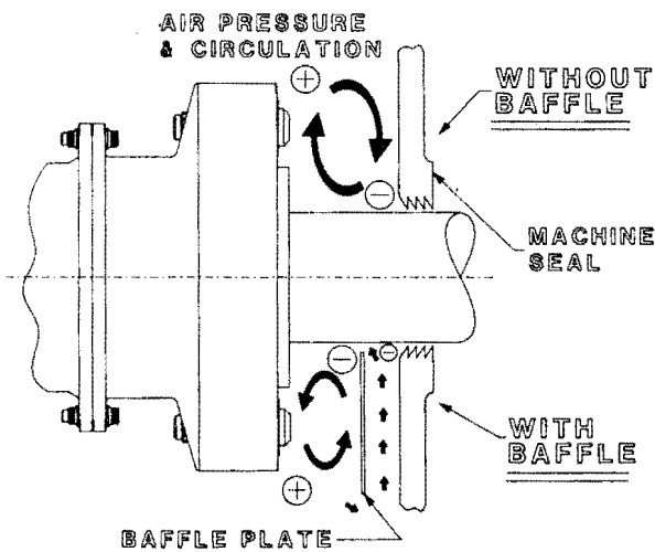
Figure 65. Baffle Plate.
