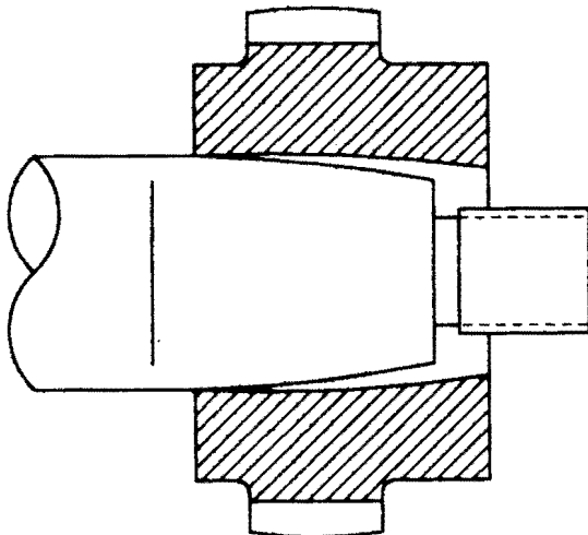
Figure 58. Result of Taper Mismatch.
