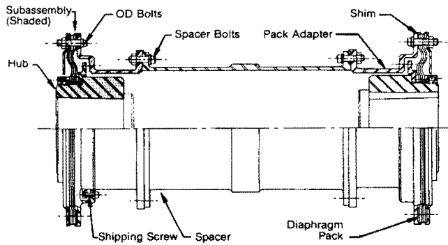
Figure 32. RM Series (reduced moment).
