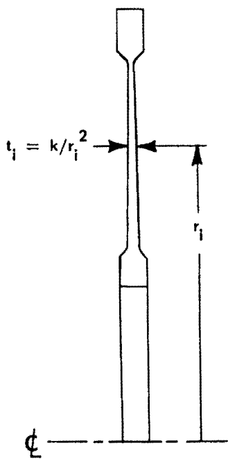
Figure 24. Contoured Diaphragm Shape.
