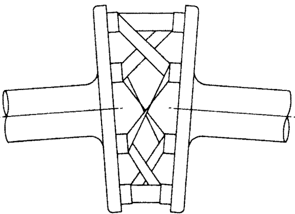
Figure 12. Disc Coupling.
