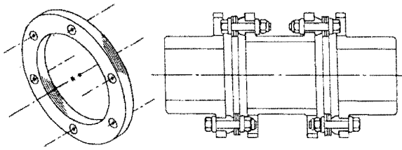
Figure 20. Disc Type Coupling.
