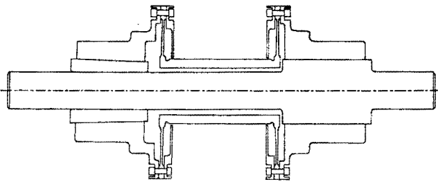
Figure 55. Coupling on Balancing Mandrel.
