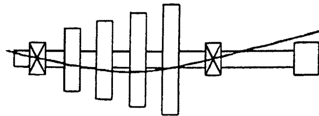
Figure 48. Machine With Long Overhang.
