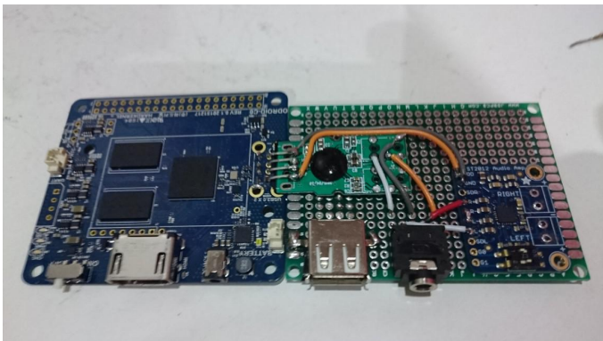
Analog multiplexer wiring
