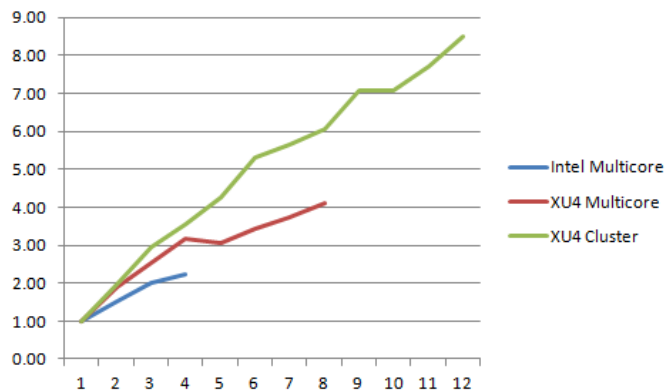
Figure 9 - Graph of performance increase of the Mandelbrot Generator as the number of cores increases
