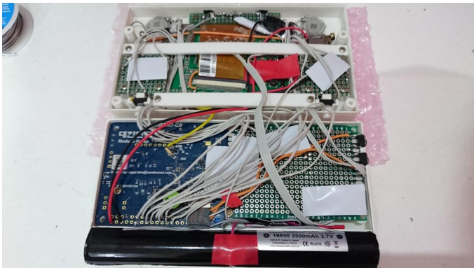
Figures 25 and 26 - All of the components are fitted into the case before closing
