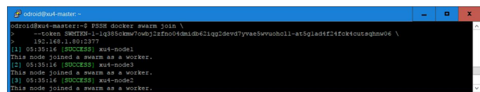
Figure 4 – Running the “docker ps” command using parallel-ssh
