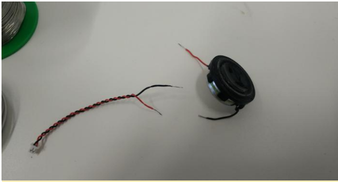
Figure 7 - Don't cut the wires too close to the speakers, in case you have to start over again. Twist the exposed wire-ends together.
