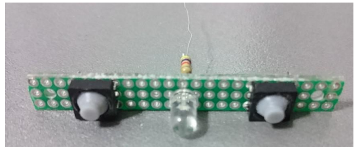
Figure 21 - Start and select button wiring
