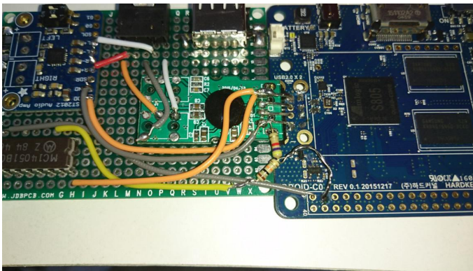
Figures 18 and 19 - Closeup of the analog multiplexer wiring
