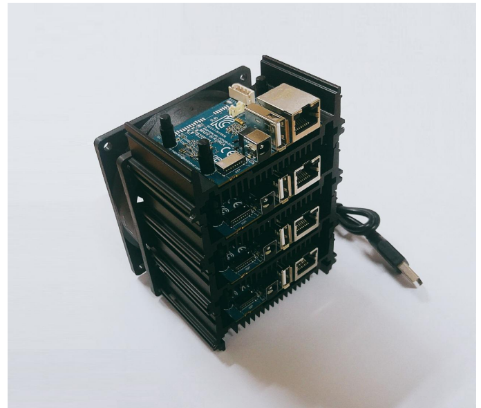
Figure 2 - The ODROID-MC1 makes an excellent swarm device
