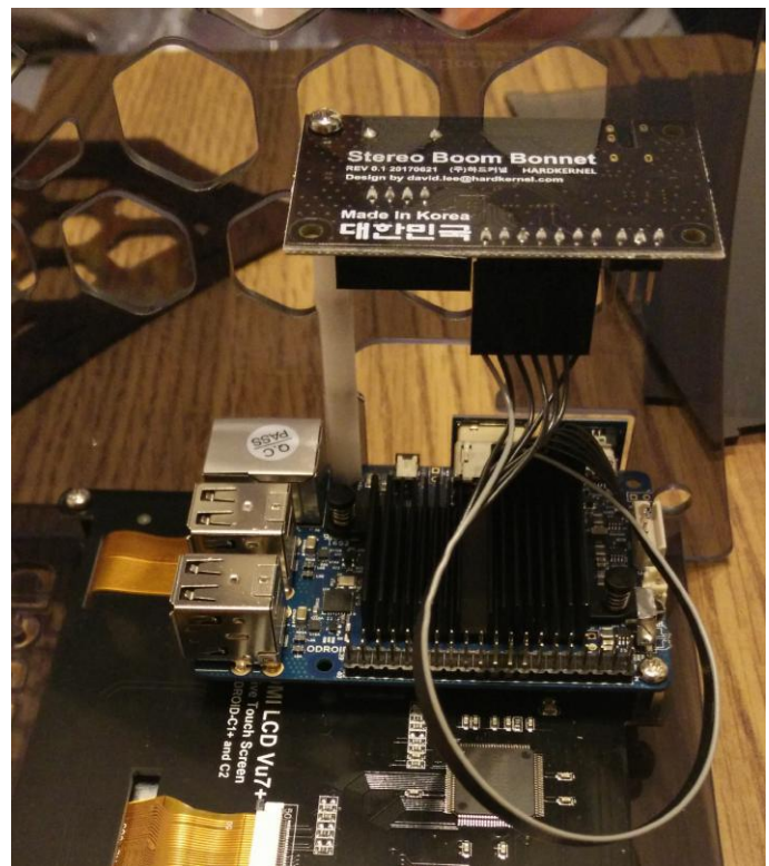
Figure 3 - Stereo Boom Bonnet connected upside down with spacers over the ODR0ID-C1+
