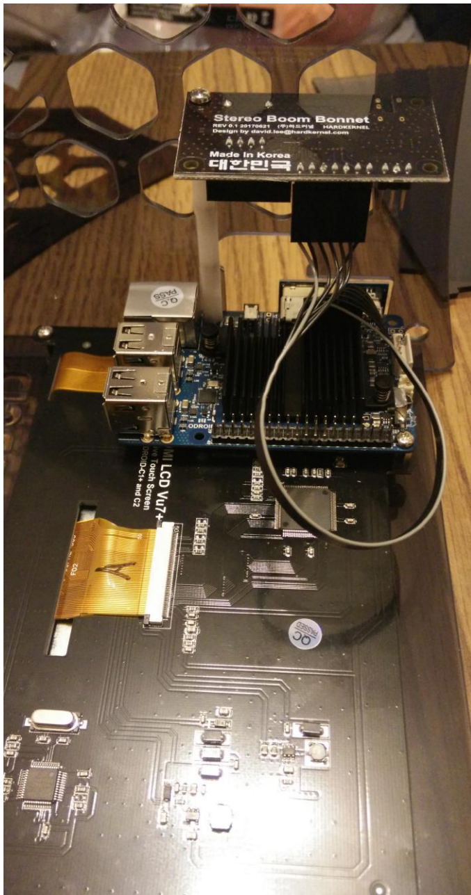
Figure 4 - I ran out of 20mm spacers and switched to 10mm. It doesn't look pretty. Please use 20mm instead. Don't be as lazy as me.
