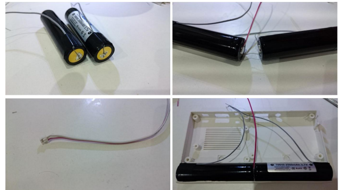
Figure 22 - Details of the battery wiring
