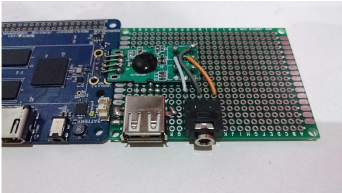
Figures 14, 15 and 16 - Wiring and soldering the components onto the extension board)
