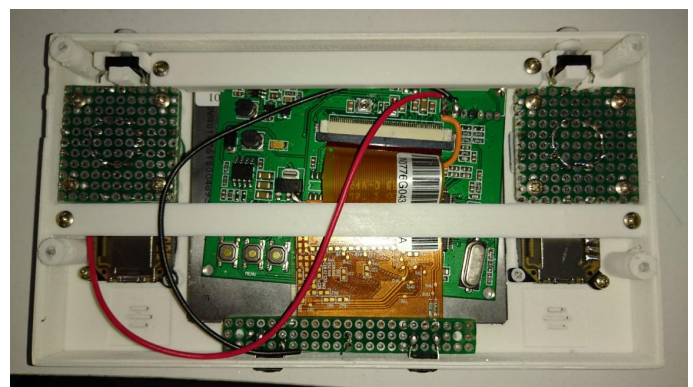
Figures 23 and 24 - Steps of the final assembly of the components inside the case
