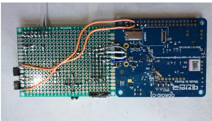
Figure 20 - Volume button wiring
