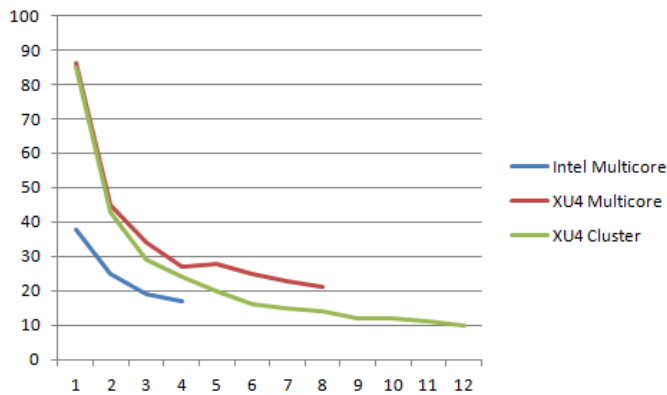
Figure 8 - Graph of the execution time of the Mandelbrot Generator as the number of cores increases
