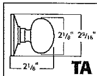
U.S. Lock's Plymouth Design
