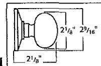
TA KNOB DESIGN
