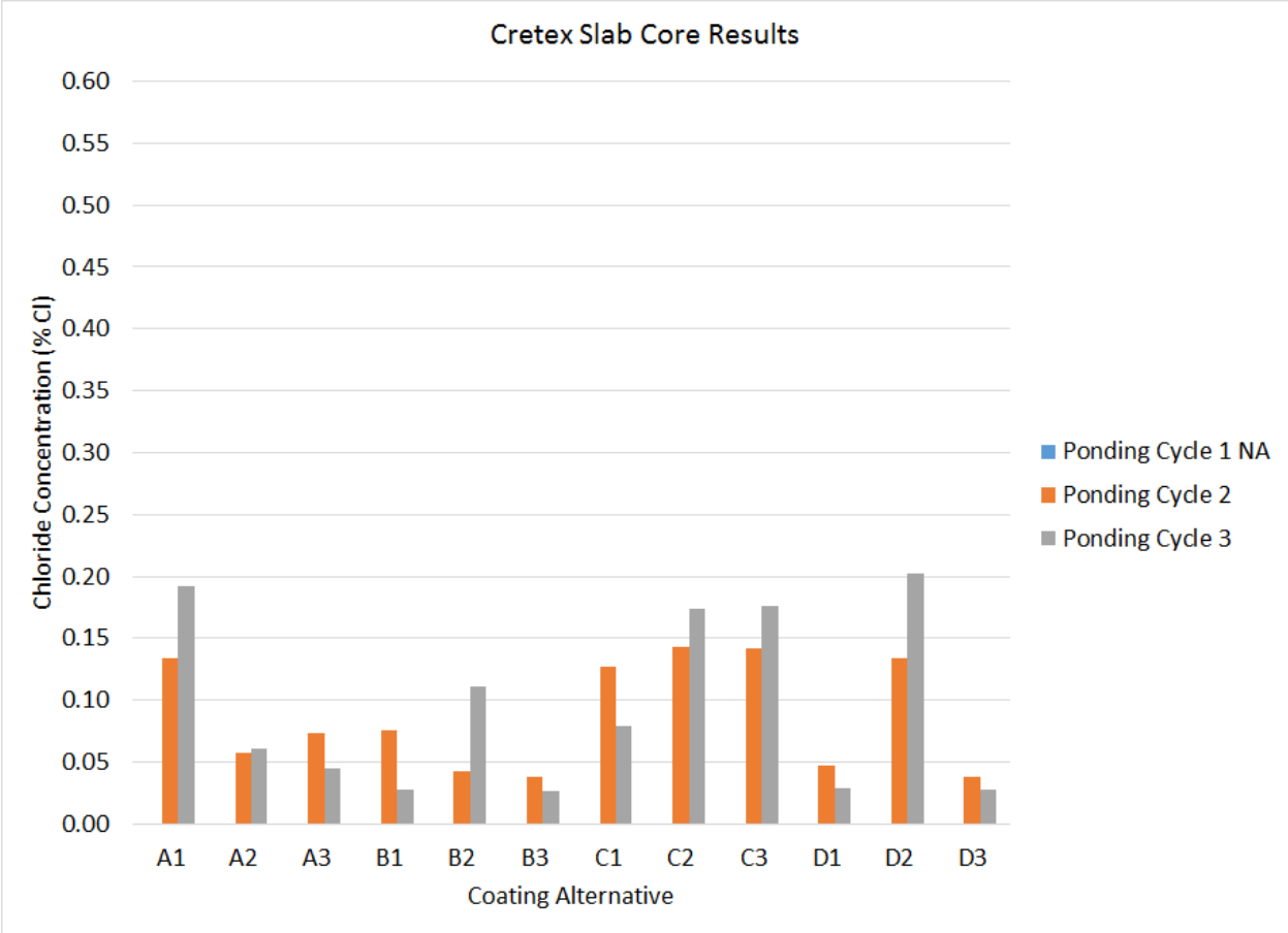
Figure 6. Chloride test results for the Cretex Slab
