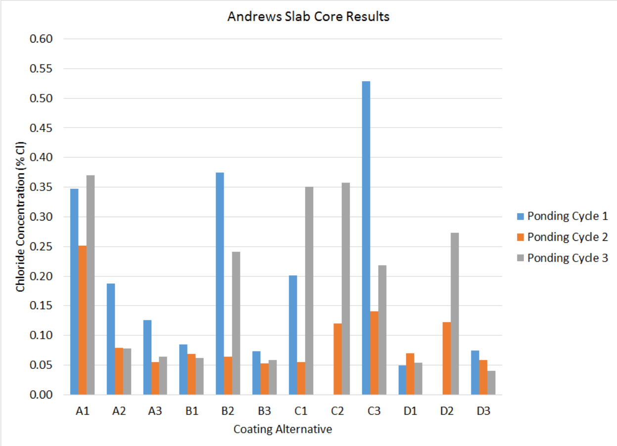
Figure 4. Chloride test results for the Andrews Slab
