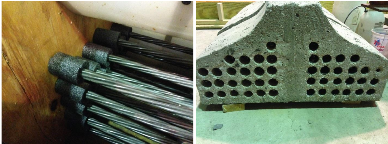
Figure 78. Bar knockout using pipe insulation cut to 2 in. lengths
