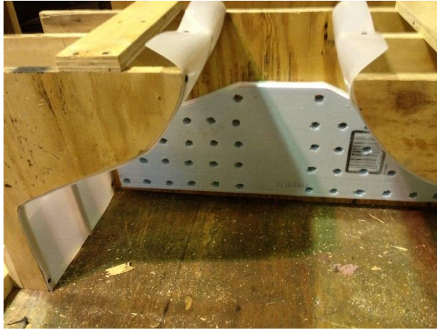
Figure 74. Single Blockout formed with 1 in. foam
