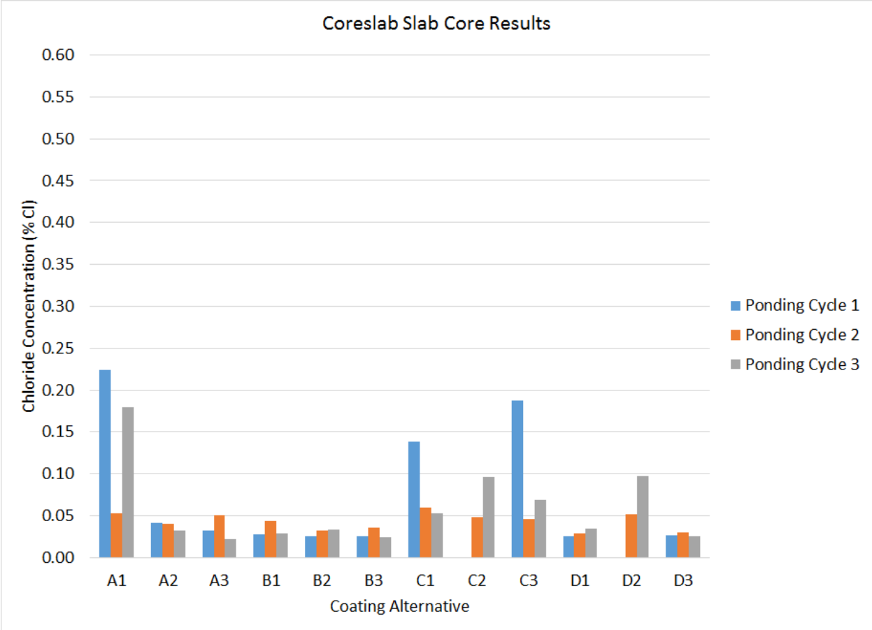
Figure 5. Chloride test results for the Coreslab Slab
