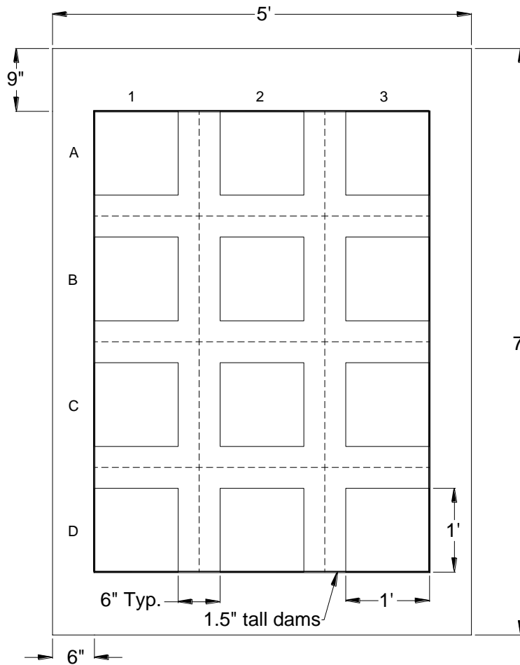
Figure 1. Dimensions of laboratory slabs for ponding tests
