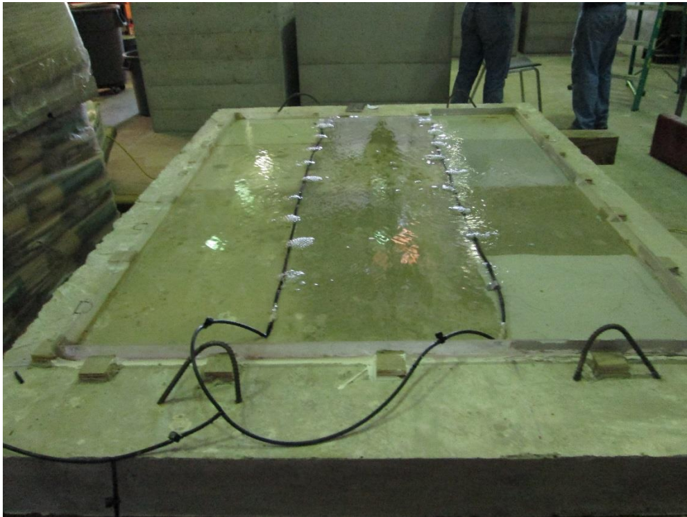
Figure 3. Laboratory specimens ponded with 3% chloride solution prior to being covered
