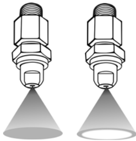
Figure 9-4: Solid and hollow core nozzles.
