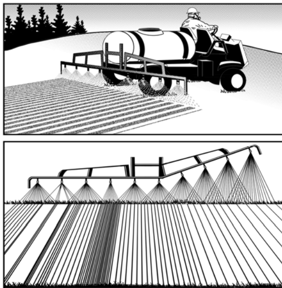
Figure 9-5: Improper boom height and clogged or worn nozzles can result in uneven application of pesticide and poor control
