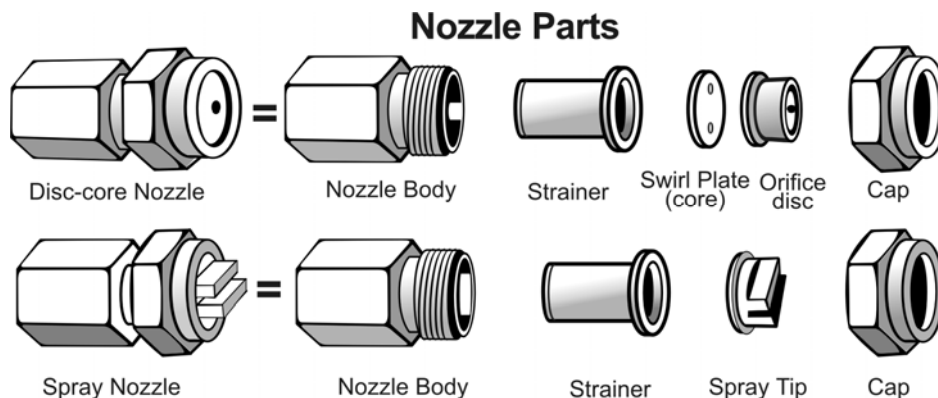
Figure 9-2: Parts of typical nozzles.
