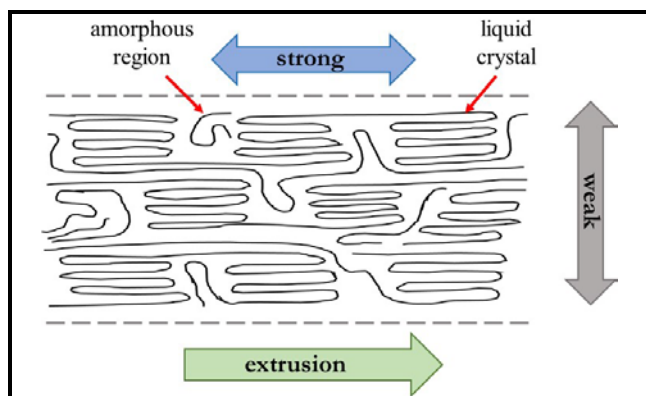
Figure 15: Extrusion process and LCP alignment. During extrusion, polymer chains become aligned in the extrusion direction while maintaining liquid crystalline regions. The result of extrusion is increased strength of the LCP monofilament fiber. (Adapted from [22]).
