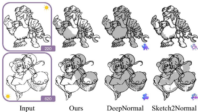
Figure 4: Comparisons with previous works DeepNormal [13] and Sketch2Normal [31] with lighting depth “2” - in the plane (side lighting). The little sun denotes the lighting direction.
