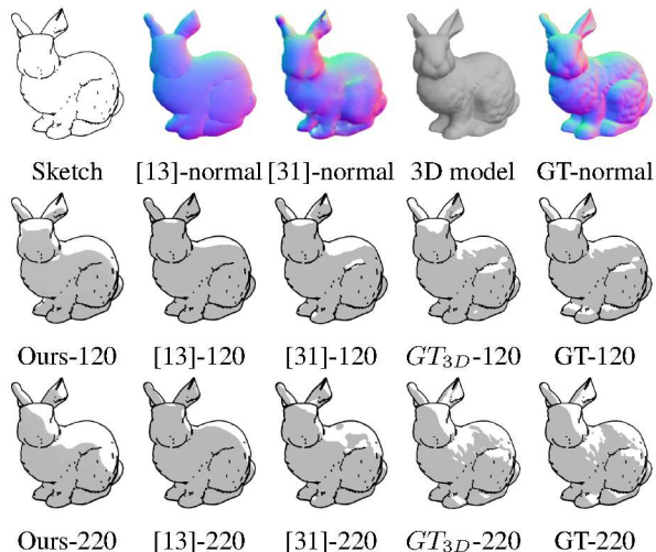
Figure 6: Comparisons between ground truth (GT), our approach, DeepNormal [13], and Sketch2Normal [31] rendered with a 3D bunny, with lighting depth “2”. “120”: top, side lighting. “220”: upper right, side lighting. “ GT_{3D} ”: rendered from commercial 3D software. “GT”: rendered from its normal map.
