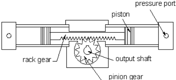
Figure 1.13 Rack and rotary actuator
