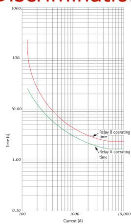
Figure 9.3: Relay characteristics for different settings
