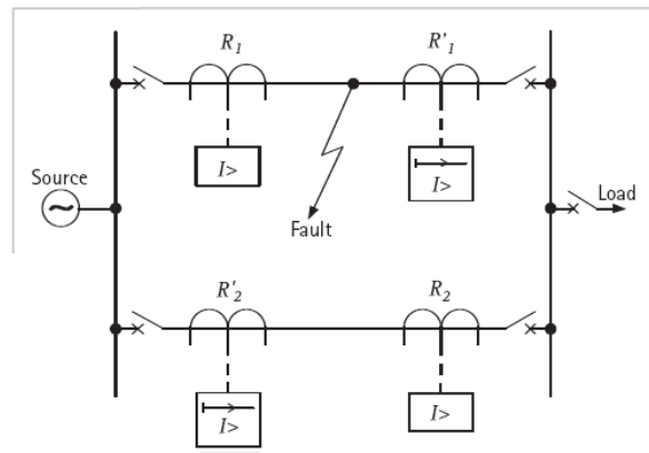
Figure 9.13: Directional relays applied to parallel feeders
