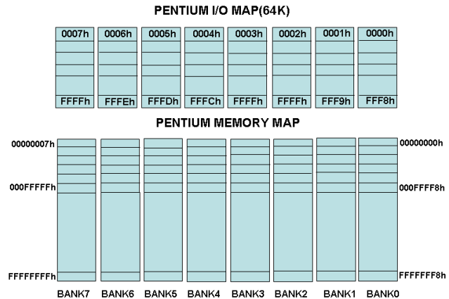
PENTIUM ADDRESS SPACE
