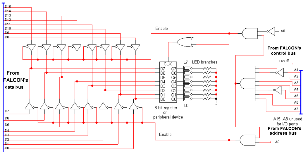
A Data Bus Multiplexer for an 8-bit Peripheral using address DCh and DDh.
