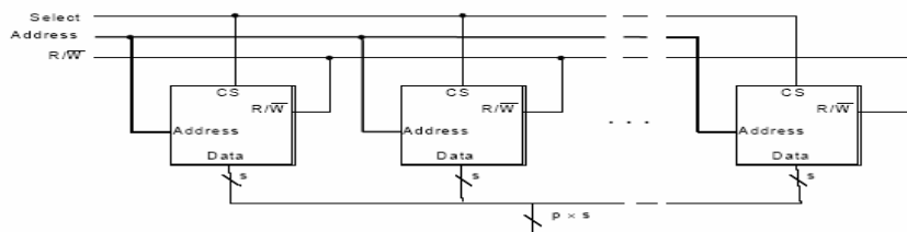
P chips expand word size from s bits to p x s bits.
