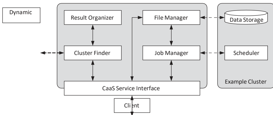
FIGURE 3.5 CaaS Service design.
