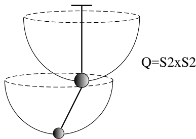
Figure 2.1: Double pendulum configuration space.
