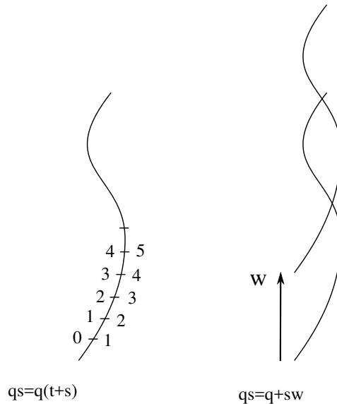
Figure 3.4: Proper time rescaling vs spacetime translation.
