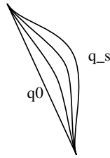
Figure 2.2: Schematic of a 1-parameter family of curves.
