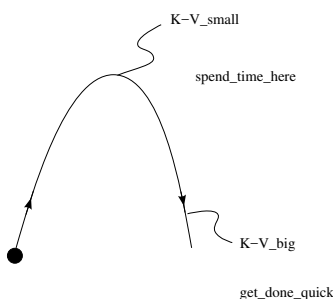
Figure 1.2: A particle’s “lazy” motion minimizes the action.
