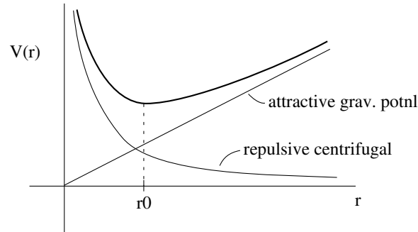
Figure 3.1: Potential function for disk pulled by gravitating mass.
