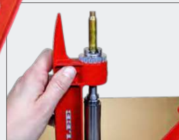
BREECH LOCK RAM PRIME
