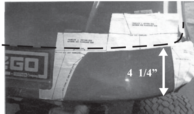
Step 3: Align template "C" with template "A & B" and 1/8" below the body line as shown above. Be sure that the outside corner where "B" & "C" meet is not more than 4 1/4" above the bottom edge of the body.
