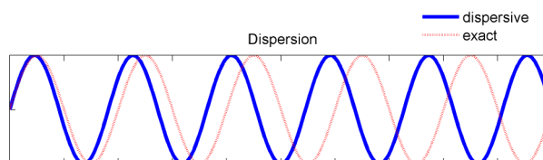
Figure 3: Illustration of pure numeric dispersion effect on a single sinusoid, as it propagates along the spatial domain. Both exact and simulated dispersive waves start in phase; however, the phase of the dispersive wave leads the exact wave over time, but its amplitude is unaffected.
