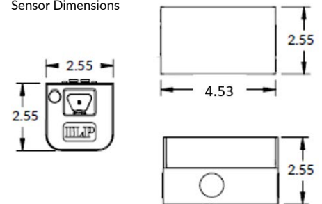
Sensor Dimensions
