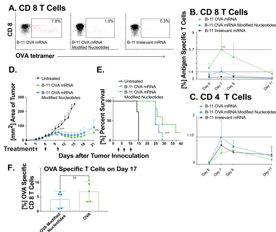
Figure 3. C57Bl/6 mice ( n = 7 ) were immunized with mRNA LNPs ( 10 \mu\text{g} mRNA per mouse in 100 \mu\text{L} of PBS; the mRNA is either unmodified or completely substituted with 5-methylcytidine (5mC) and pseudouridine ( \psi )), and subsequently, mice were bled at specific time points. The red blood cells were lysed, and the monocytes were stained with tetramer, live–dead stain, and CD4 and CD8 antibody conjugates. (A) Representative FACS profiles of mice treated with the indicated conditions. The CD8 T cell response in peripheral blood is much stronger from unmodified mRNA LNP vaccines. (B) The percentage of OVA specific CD8 T cells peaks at day 7 after subcutaneous injection. Compared to unmodified mRNA, the substitution with 5mC and \psi induces an immune response only slightly higher than in the group treated with irrelevant control mRNA LNPs. mRNA coding for \beta -galactosidase was used as the irrelevant control (** P < 0.01 by the ordinary one-way ANOVA Bonferroni's multiple comparisons test). (C) No significant increase in circulating antigen specific CD 4 T cells could be detected. (D) mRNA LNP formulation B-11 induces potent in vivo antitumor immunity. Mice (C57Bl/6J, n = 10 for the control group and n = 5 for the treated mice) were injected subcutaneously in the upper back with 1 \times 10^5 B16-OVA melanoma cells on day 0. Treatment began when tumors were clearly visible in all mice (day 3) with LNP formulation B-11 containing OVA mRNA either modified or unmodified (days 3, 6, and 10, 10 \mu\text{g} of total mRNA per mouse and injection). Both treatment groups slow down tumor growth after the second treatment and shrink the tumor after the third treatment. Mice that reached the maximal allowed tumor area of 250 \text{ mm}^2 , or that developed ulceration, were euthanized and recorded as having tumor areas of 250 \text{ mm}^2 (** P < 0.01 , *** P < 0.001 , as compared with the untreated control group, two-way ANOVA with Bonferroni posthoc). (E) Overall survival is increased for both treatment groups. Statistical analysis was done using a log rank analysis (*** P < 0.001 , as compared with the untreated control group, Mantel Cox test). The two mRNA treated groups are not significantly different). (F) The percentage of SIINFEKL specific CD 8 T cells that were analyzed on day 17; the difference in CD 8 T cells was not statistically significant.
