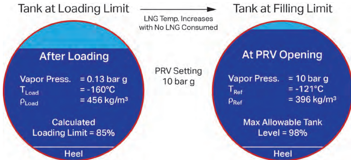
Figure 2. Typical Pressurized Tank Loading Limit
