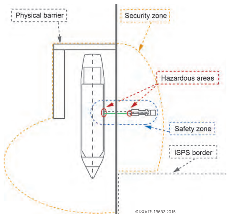
Figure 9. Example of Safety and Security Zones
