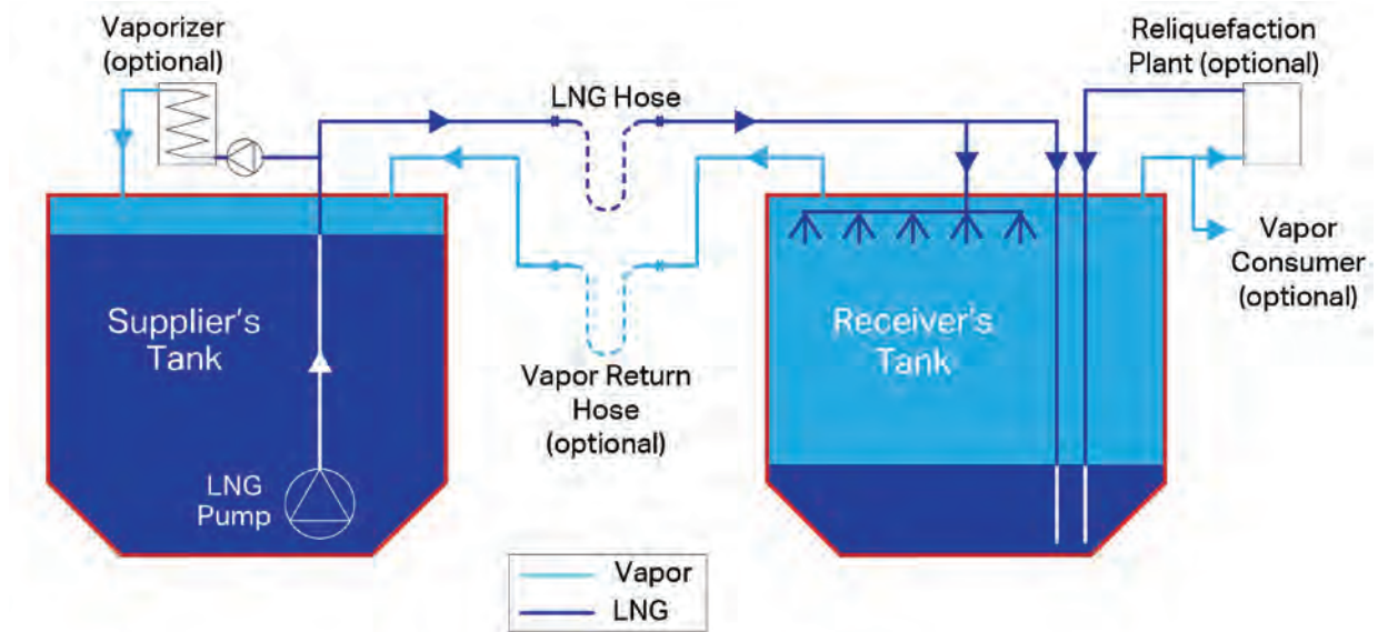
Figure 6. Typical Arrangement of Bunker Piping and Connections
