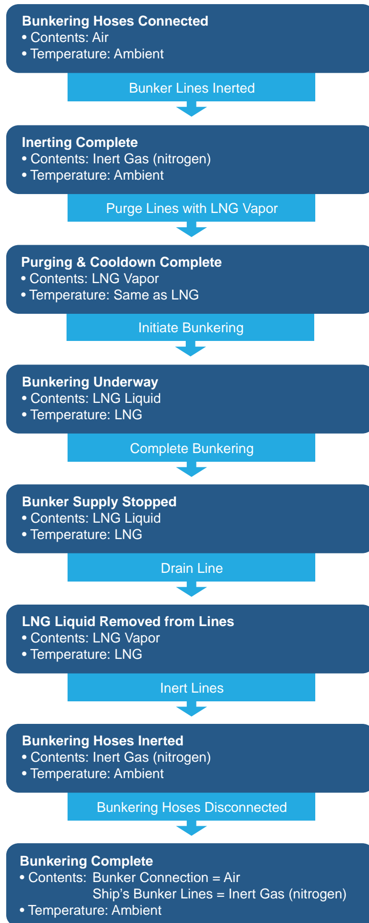
Figure 3. Inerting and Purging Sequence of LNG Bunker Hose and Piping
