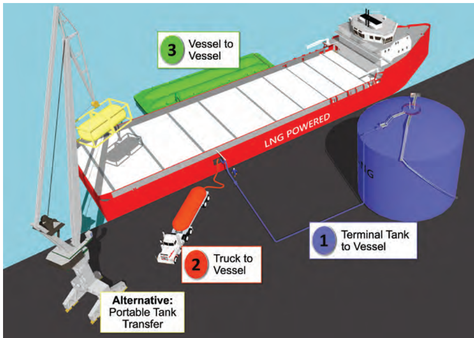
Figure 7. Typical Methods of Bunkering a Gas Fueled Ship
