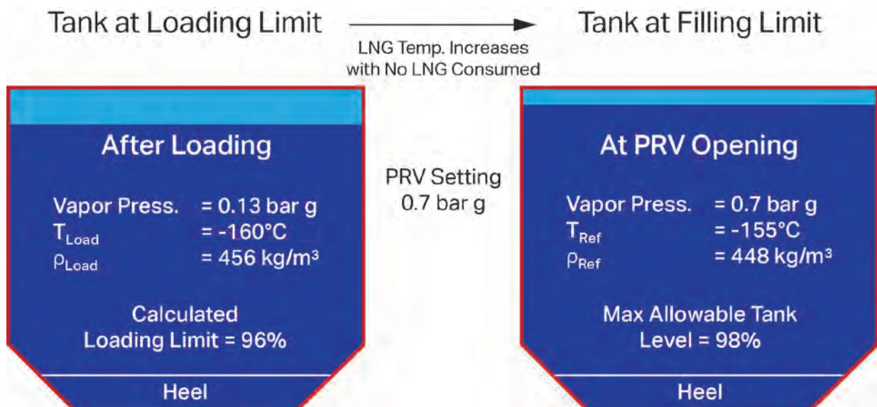
Figure 1. Typical Atmospheric Tank Loading Limit
