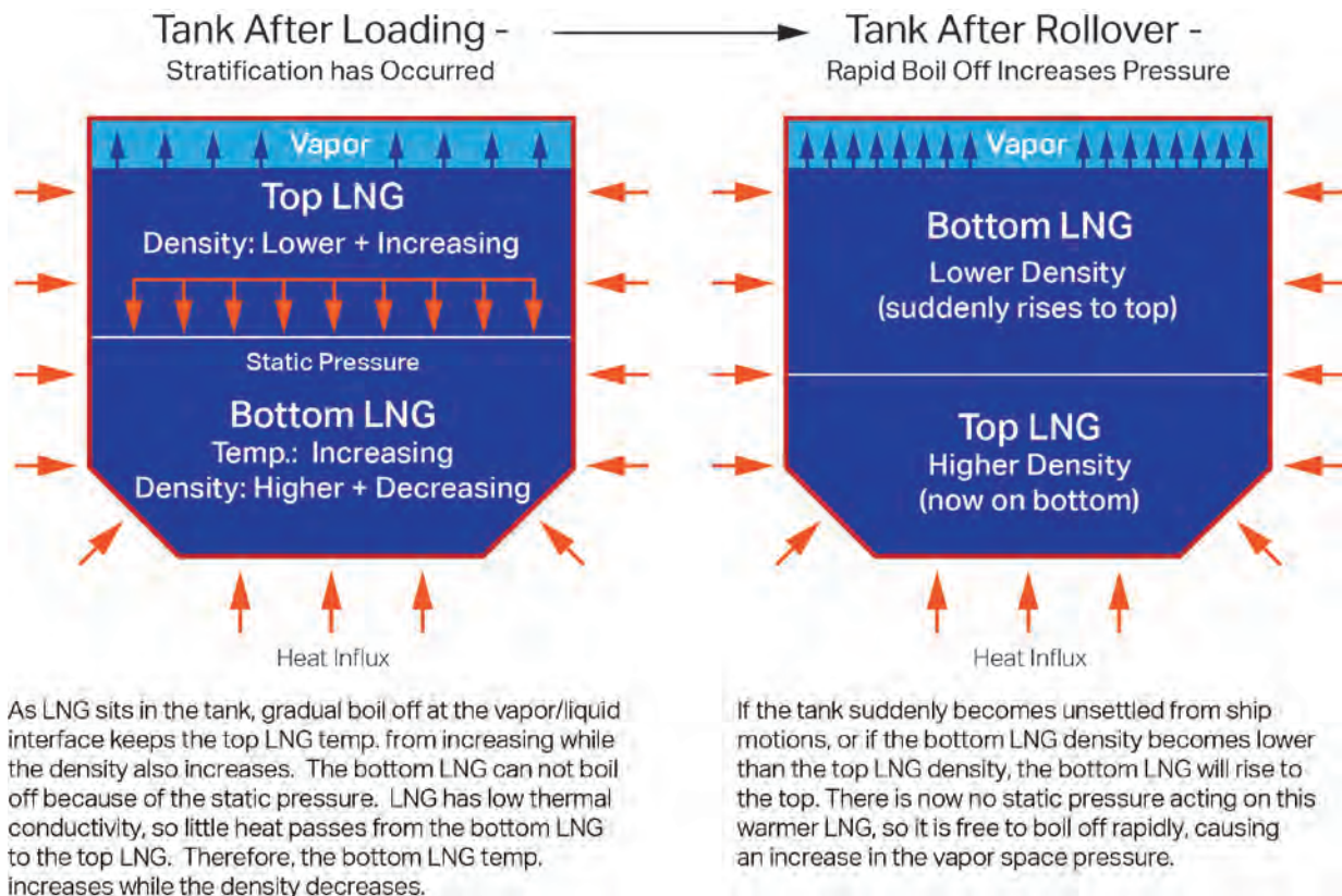
Figure 5. Rollover After Stratification
