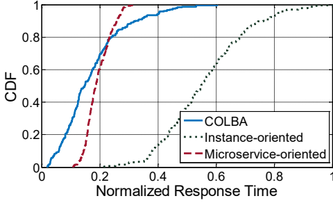
Fig. 10. CDF of response time, COLBA vs. baselines.
