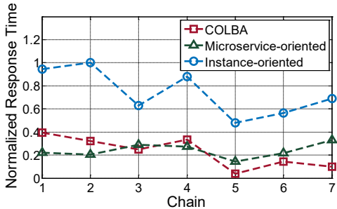
Fig. 11. The normalized response time of COLBA against instance-oriented and microservice-oriented solutions.
