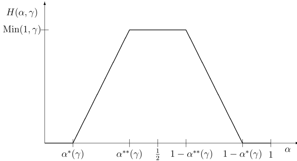
Figure 3: The density-of-equilibria function H(\alpha, \gamma) .
