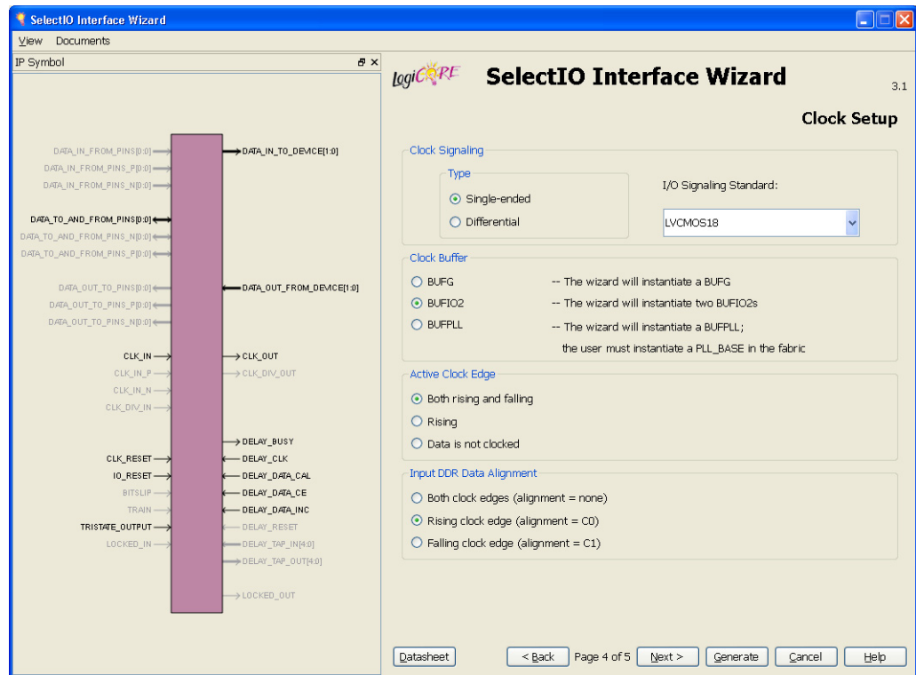
Figure 5-4: Clock Setup - Page 4
