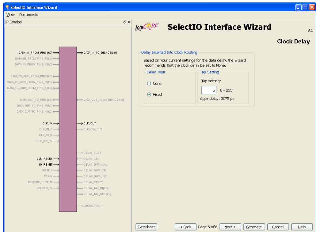
Figure 5-5: Clock Delay - Page 5
