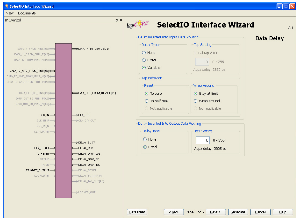
Figure 5-3: Data Delay - Page 3
