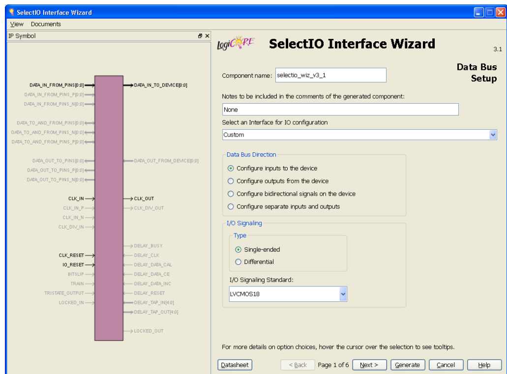
Figure 5-1: Main Screen- Data Bus Setup - Page 1
