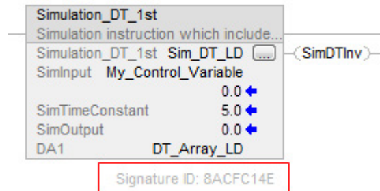
Ladder editor
