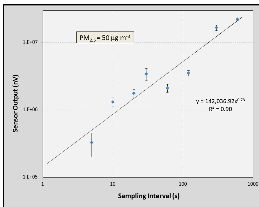
Fig. 3. Variation of the Shinyei sensor readings with sampling interval at a fixed concrete dust concentration ( \text{PM}_{2.5} = 50 \mu\text{g m}^{-3} ). The error bars represent the standard deviation of multiple measurements at each time interval.
