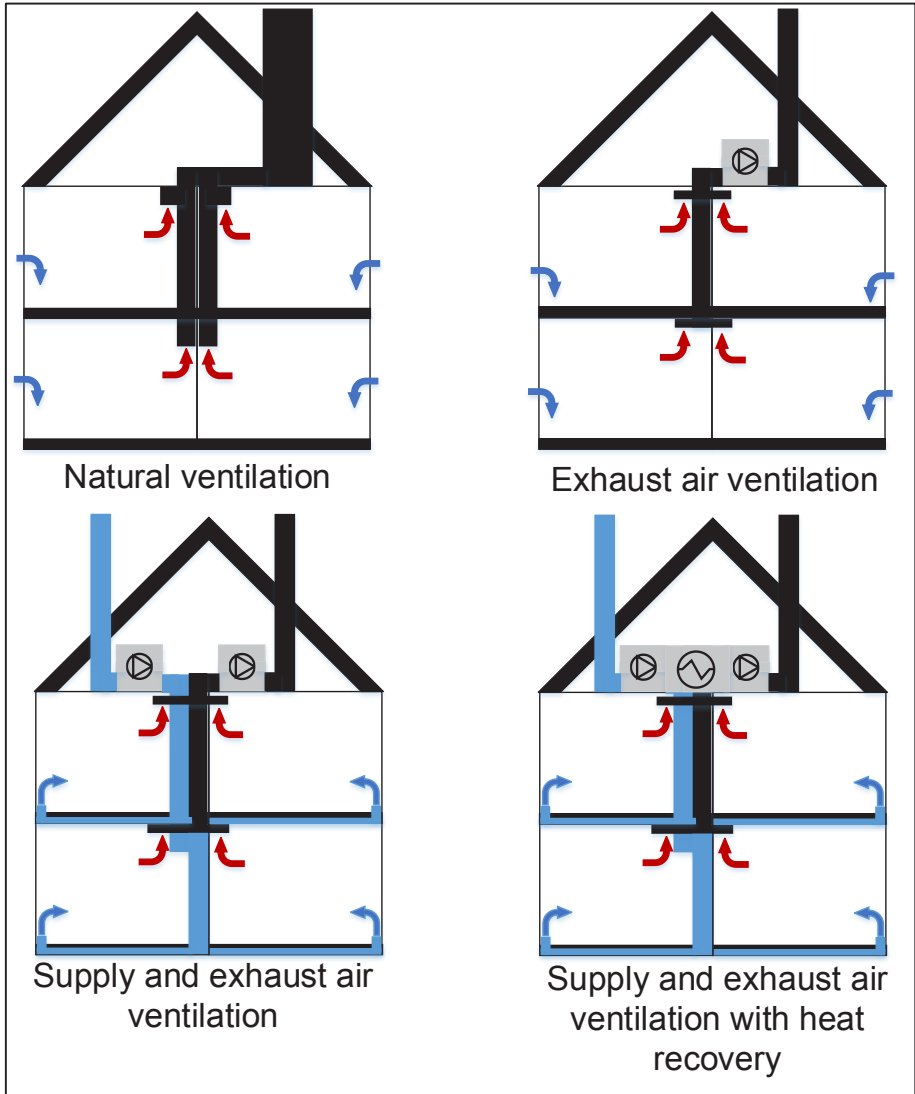
Figure 3. Different types of ventilation systems
