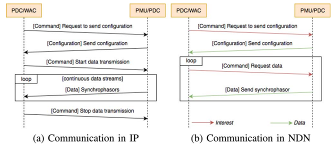
Fig. 5. Communications between PMUs and PDC/WAC.
