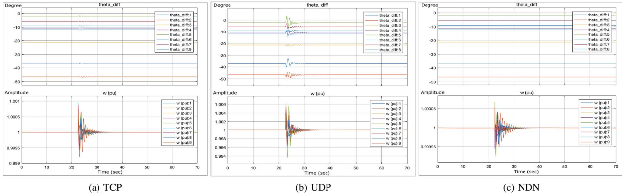
Fig. 11. Effect of IP-based (TCP &amp; UDP) and NDN-based Architecture on Grid Stability.
