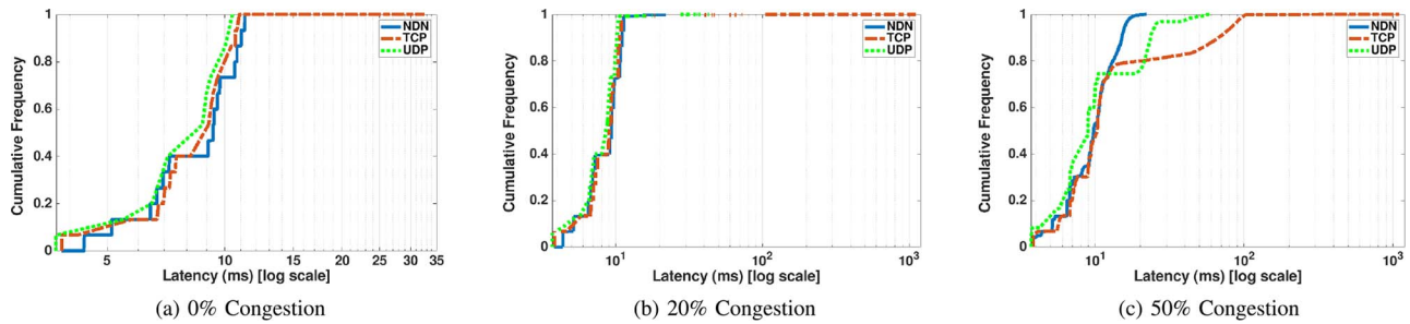
Fig. 10. Latency Comparison for Different Congestion Duration on a 300 sec Simulation.
