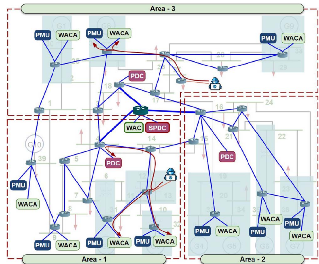
Fig. 7. Superimposed Cyber over Power System for IEEE-39.
