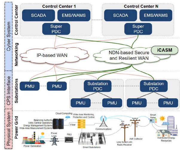
Fig. 1. IP-based and Proposed ICN-based CPS for WAMS.
