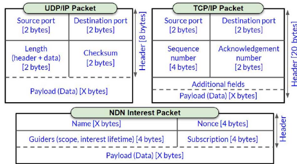
Fig. 3. Packet Schematic: UDP/IP, TCP/IP and NDN ( Interest ).
