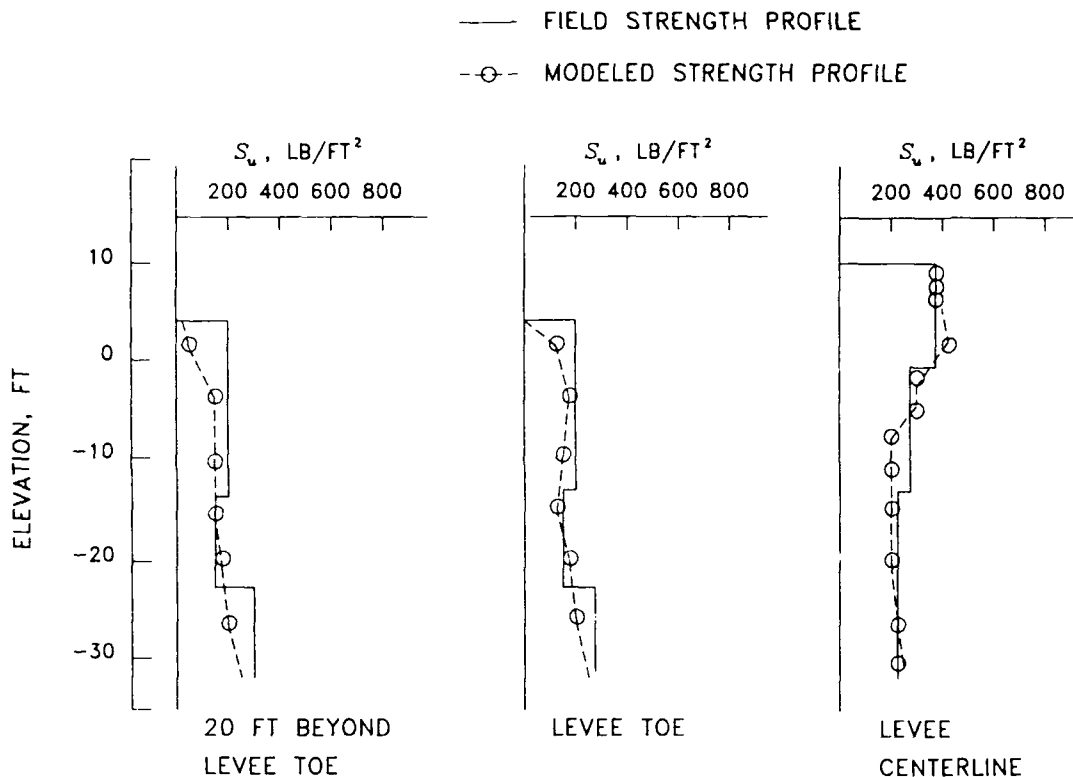
Figure 10. Comparison of design strength profile and strengths from selected elements for "weak" soil profile
