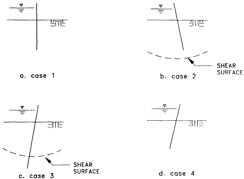
Figure 12. Different cases of levee and sheet pile stability
