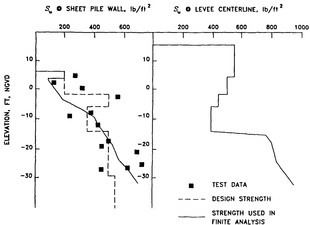
Figure 4. Comparison of design strength profile and strengths from elements at pile location
