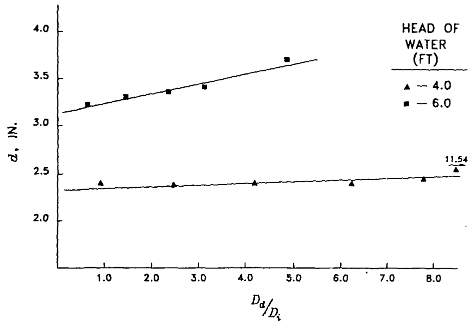
Figure 22. Movement at pile tip due to movements in foundation for the E-105 "weak" soil profile
