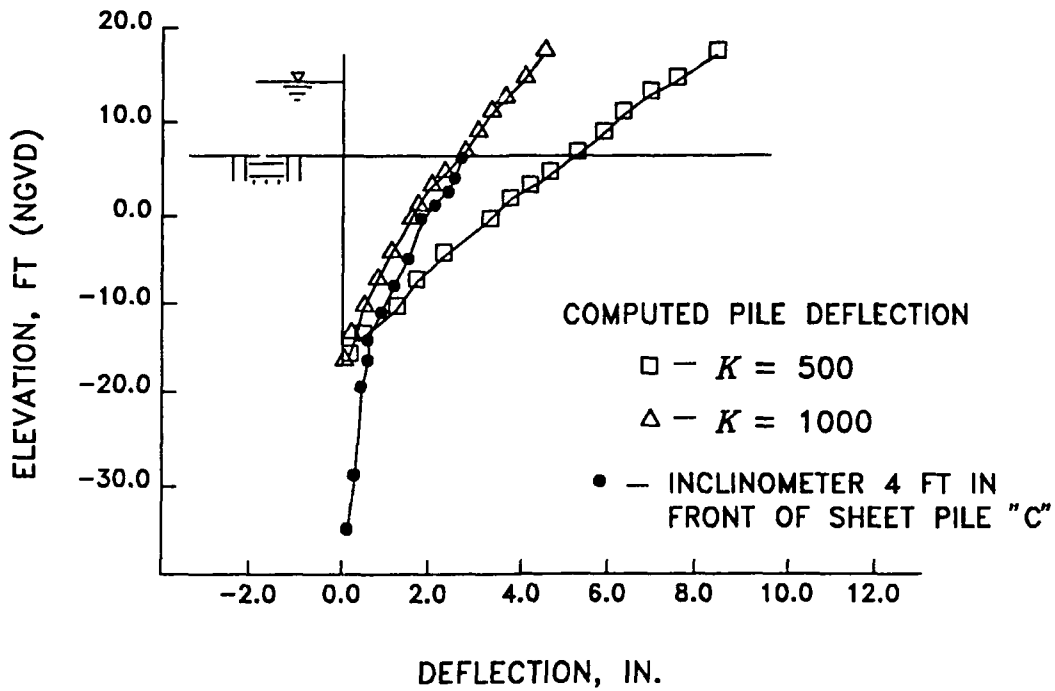
Figure 6. Comparison of computed deflection of "C" pile with displacements of inclinometer at E-99 test section
