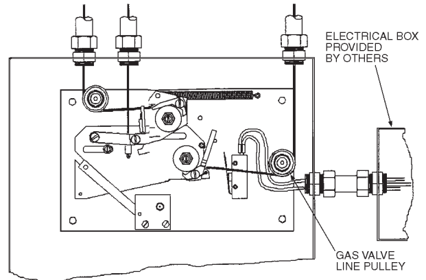
► Figure 4-34. Gas Valve / Snap-Action Switch Installation.
