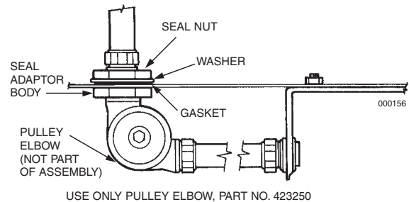
Figure 2-13b. Hood Seal Adaptor Assembly.
