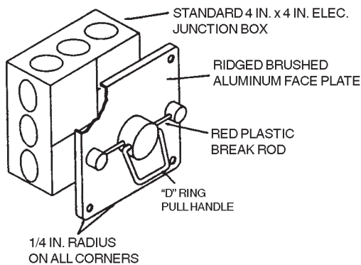
Figure 2-12. Model RPS-M Mechanical Pull Station. 002852PC
