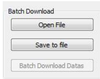
Figure 3.8 Batch Download
