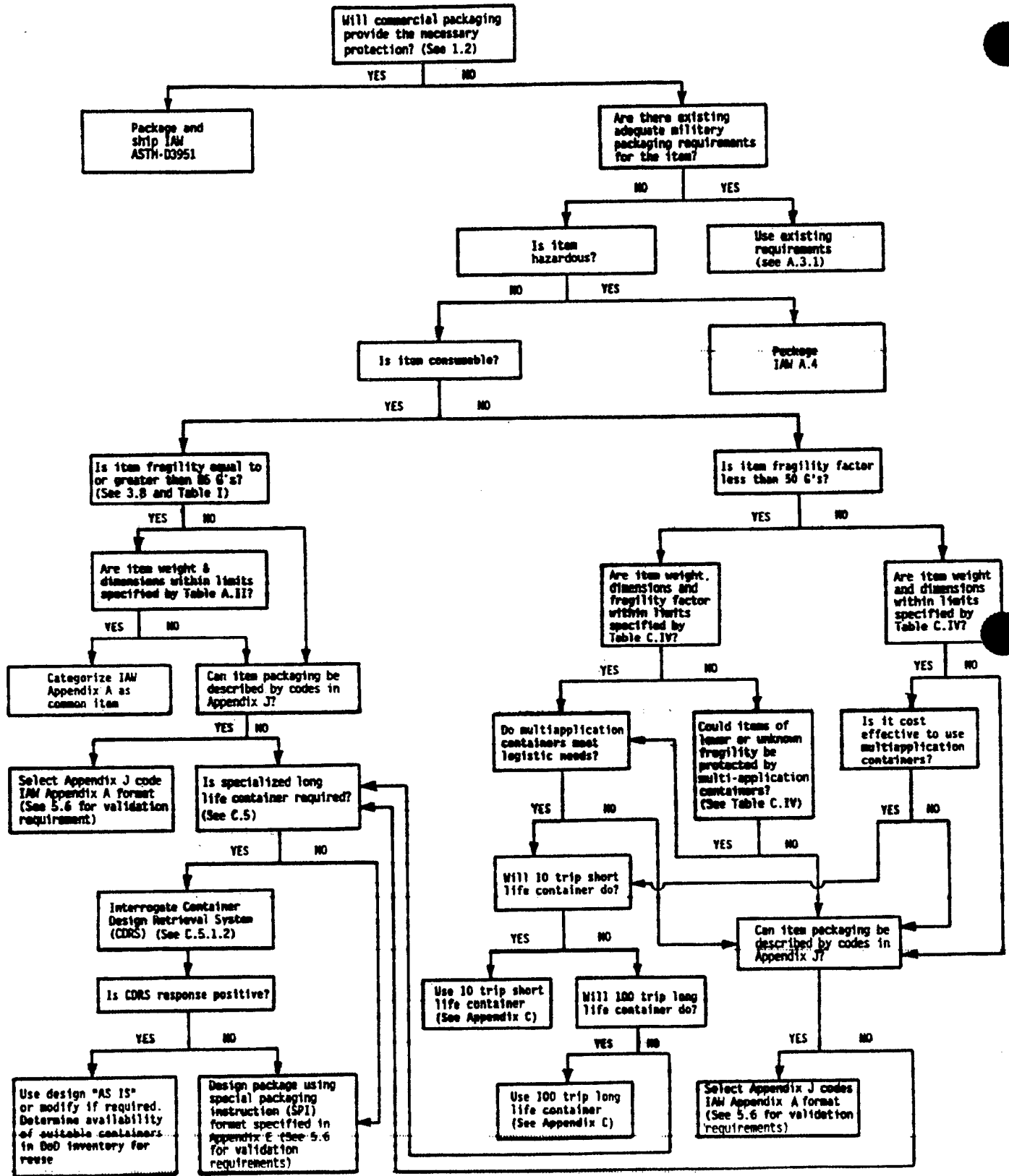
FIGURE 1. Military packaging requirements development decision chart.
