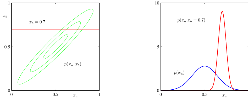
Figure 8: Left: The contours of a Gaussian distribution p(x_a, x_b) over two variables. Right: The marginal distribution p(x_a) (blue curve) and the conditional distribution p(x_a|x_b) for x_b = 0.7 (red curve). (Figure from Pattern Recognition and Machine Learning by Chris Bishop.)
