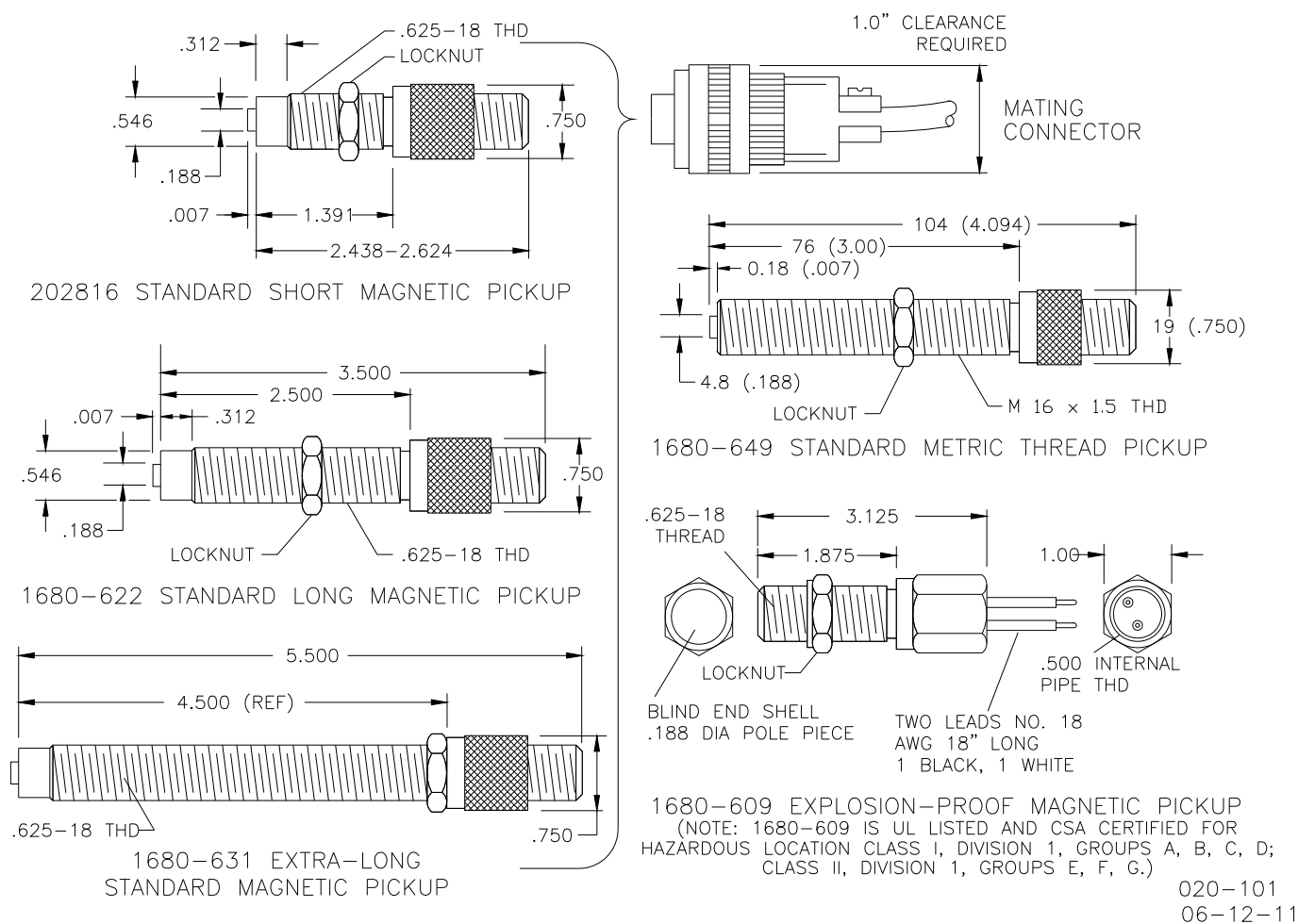
Figure 1-3a. MPU Models
