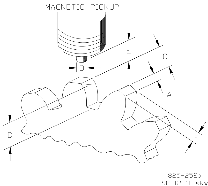
Figure 1-1. Magnetic Pickup Dimensions
