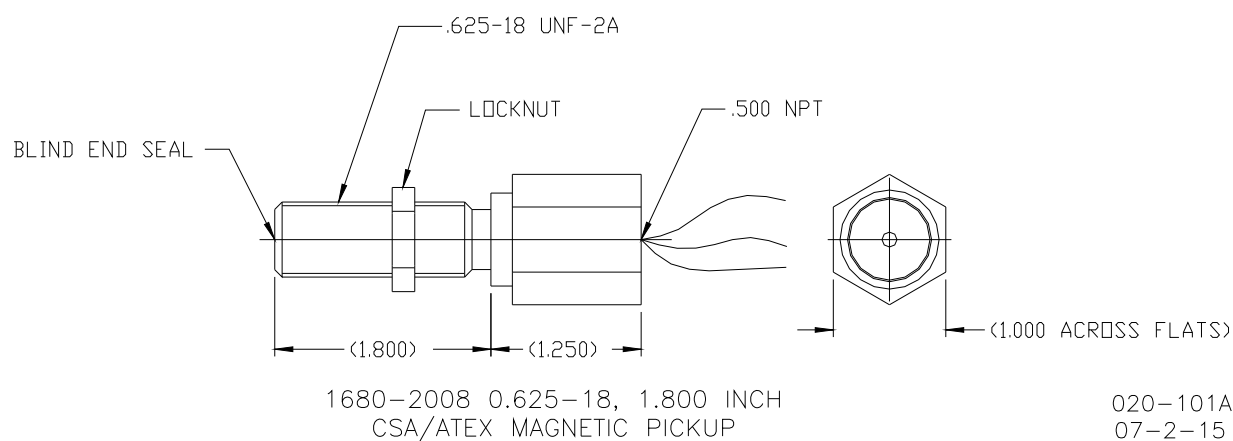
Figure 1-3b. CSA/ATEX Models (SIL 3 Models have “.SIL” at the end of the part number – Dimensions Unchanged)
