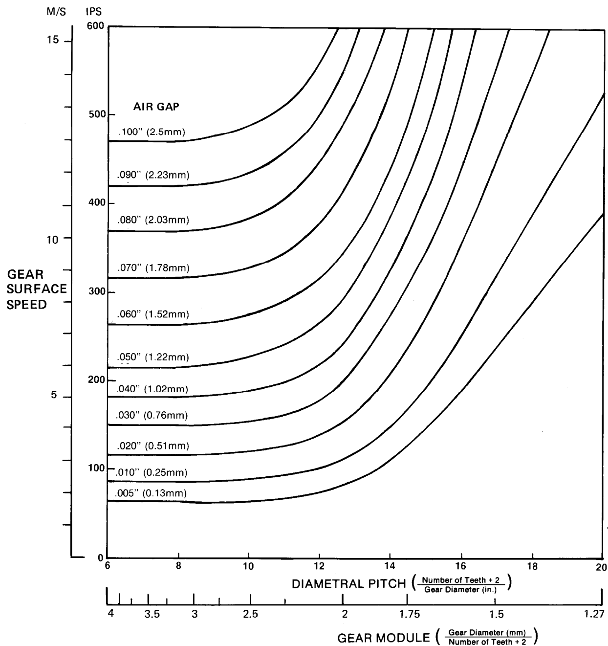
Figure 1-5. Maximum Air Gap Allowed to Provide 1.5 V (ac, rms) on EGM Control
