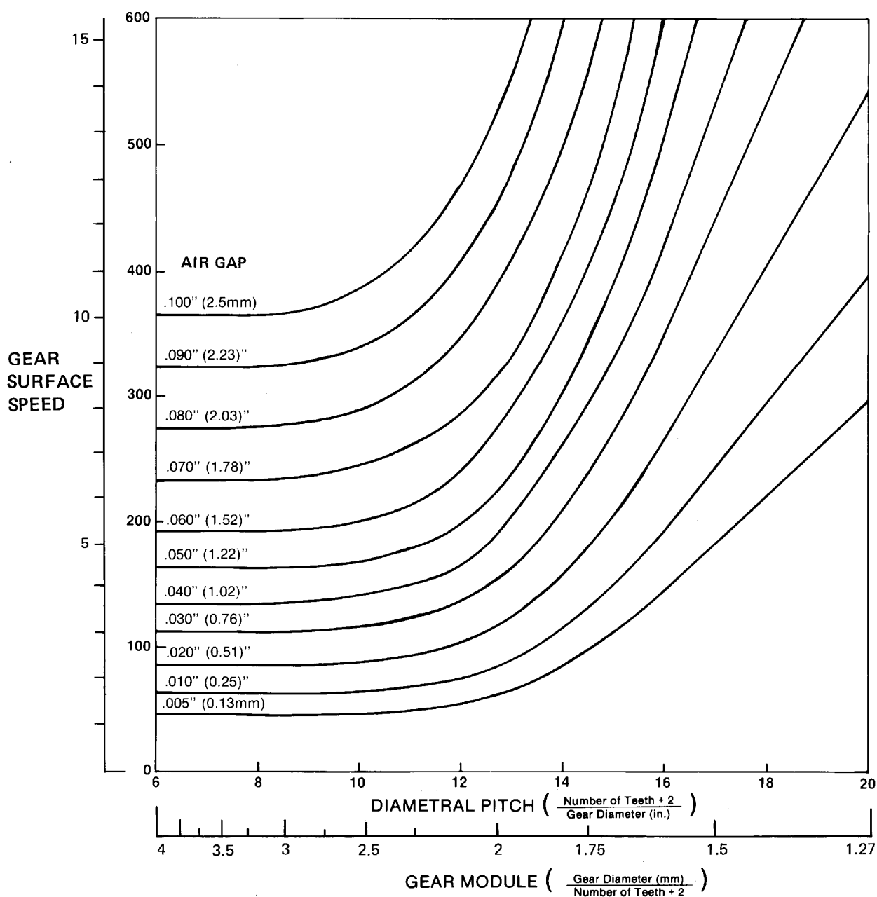
Figure 1-4. Maximum Air Gap Allowed to Provide Usable Signals for Most Electronic Controls
