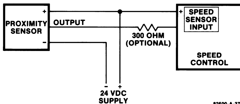
Figure 2-2. Suggested Wiring for a “Sinking” Type Proximity Switch
