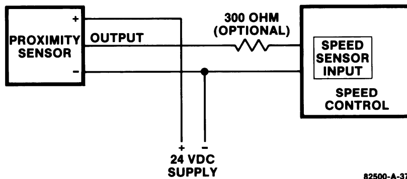
Figure 2-3. Suggested Wiring for a “Source” Type Proximity Switch
