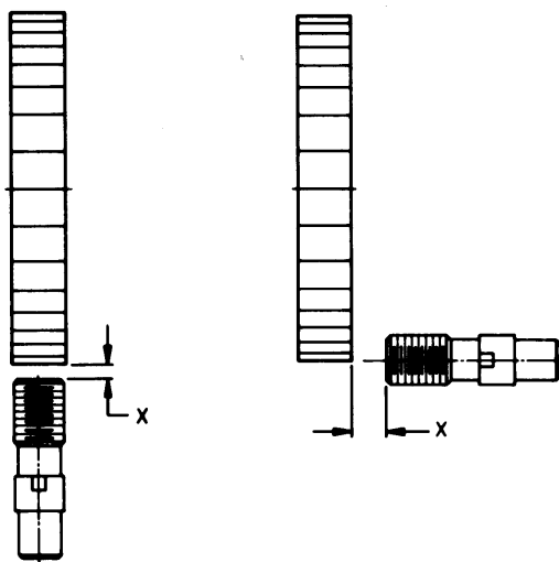
Figure 2-1. Air Gaps for Radial and Axial Sensing Proximity Switches
