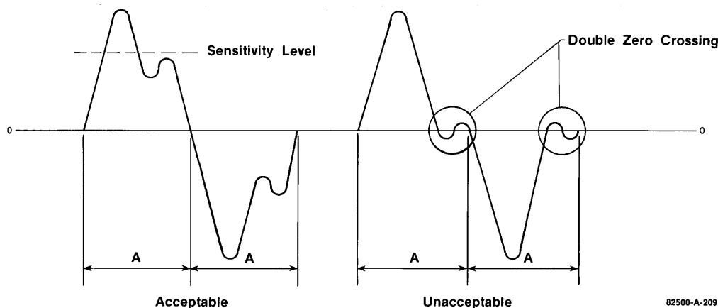
Figure 1-2. Magnetic Pickup Output Waveforms
