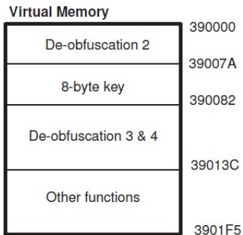
Figure: Zeus botnet (Binsalleh et al., 2010)
