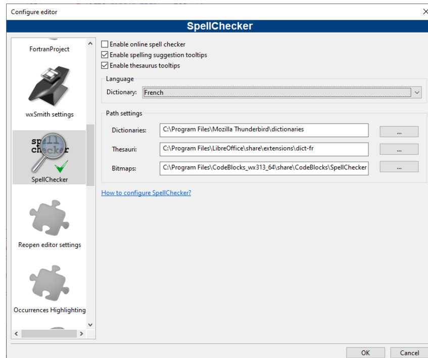
Figure 2.19: SpellChecker Configuration
