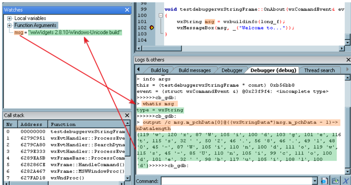
Figure 4.18: Debugger command
