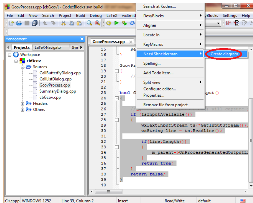
Figure 2.14: NassiShneiderman Create
