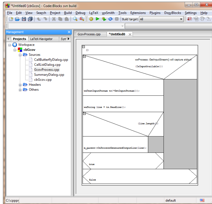
Figure 2.15: NassiShneiderman Diagram Example
