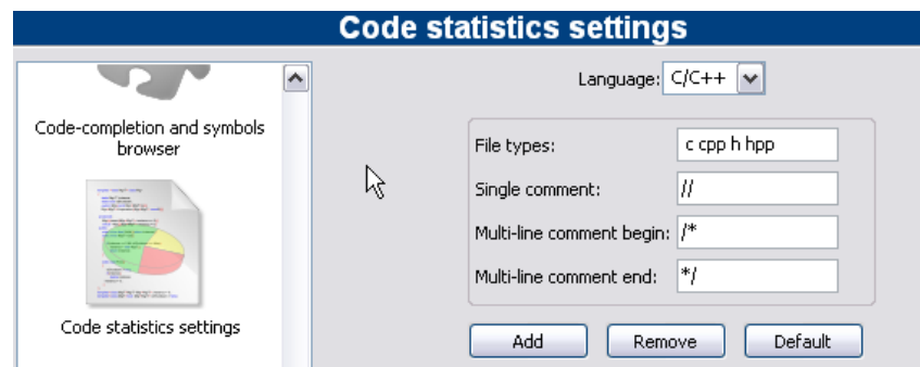
Figure 2.28: Configuration for Code Statistics
