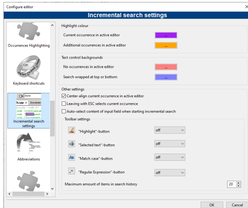
Figure 2.13: Settings for Incremental Search
