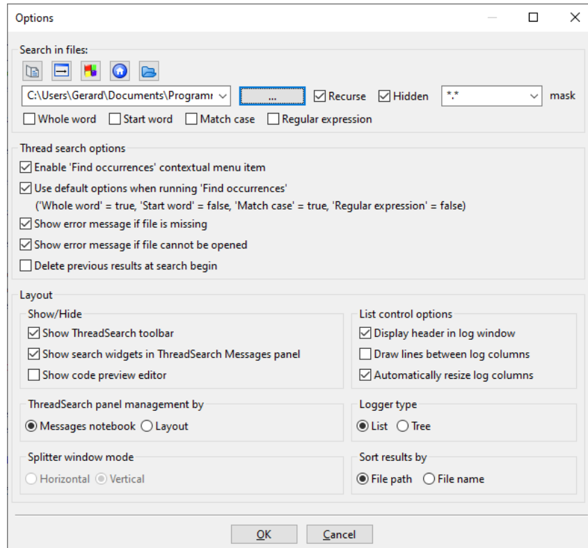
Figure 2.27: Configuration of Thread Search
