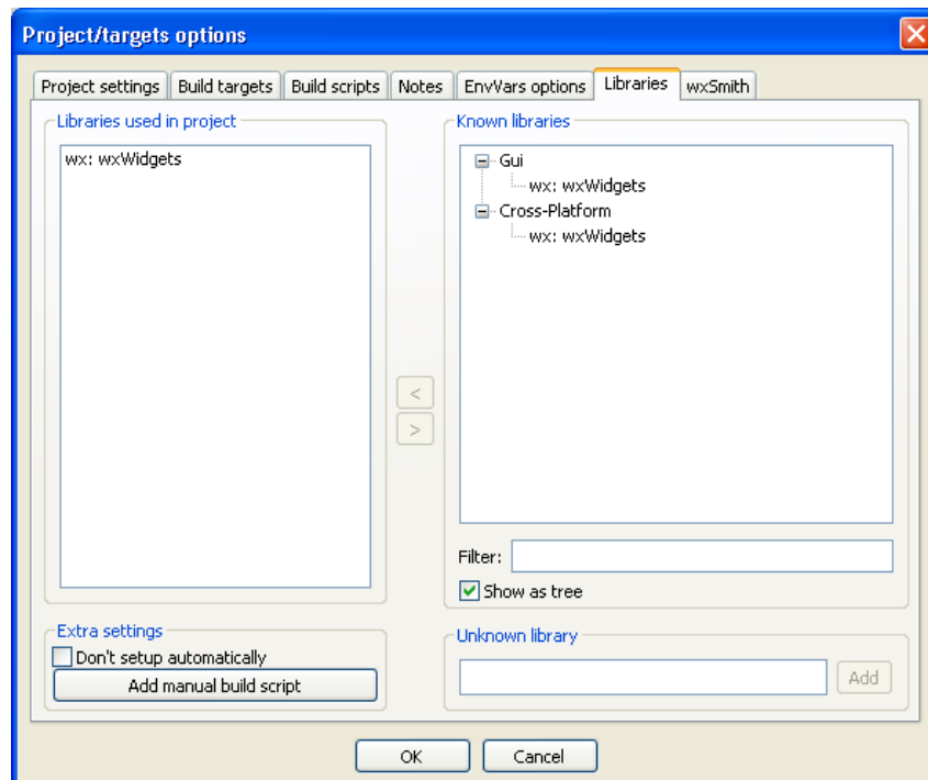
Figure 2.18: Project configuration
