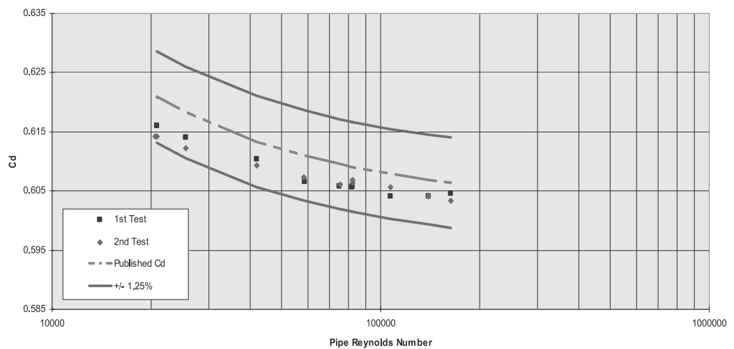
Figure 3-2: Sensor 13443 test results
