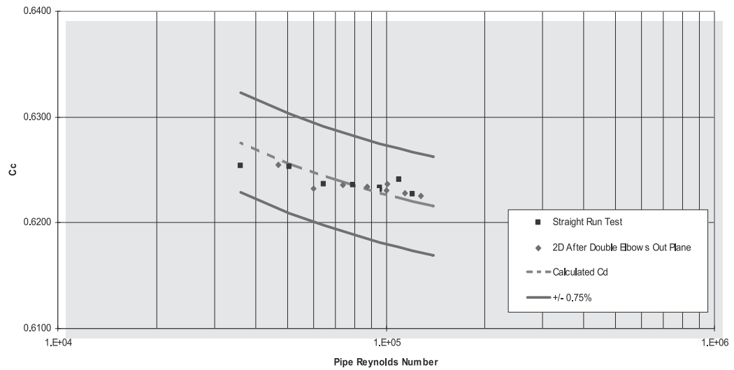
Figure 3-18: Test results for sensor 12402 in water
