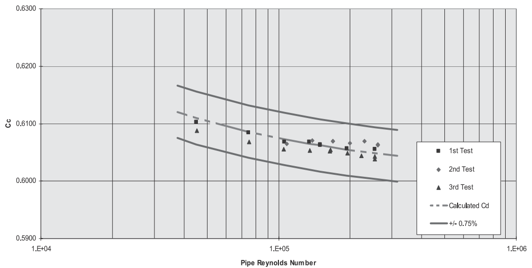
Figure 3-7: Sensor serial number 24061 test results
