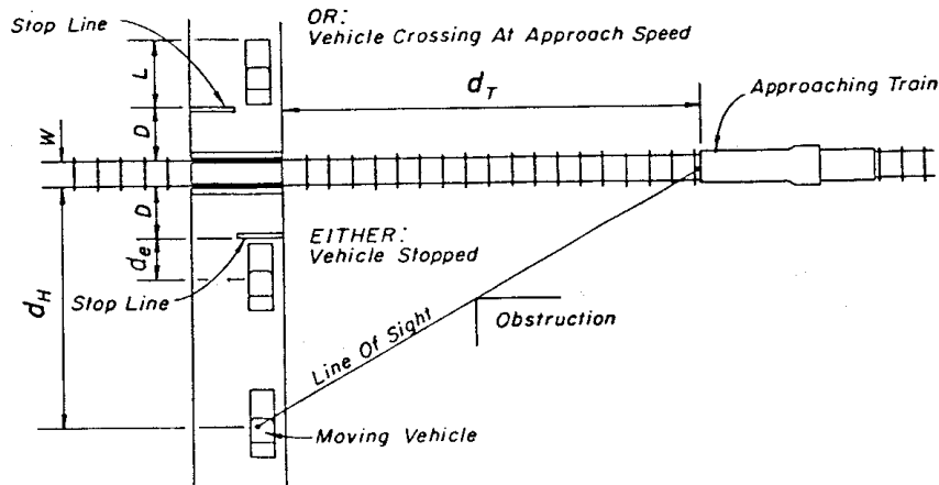
CASE A APPROACHING VEHICLE TO SAFELY CROSS OR STOP AT RAILROAD CROSSING
