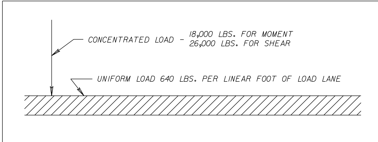
FIGURE 17 – 2 HS20-44 LANE LOADING
