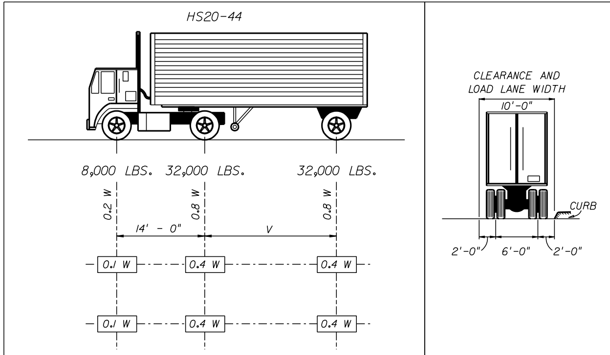
FIGURE 17 – 1 STANDARD HS20-44 TRUCKS
