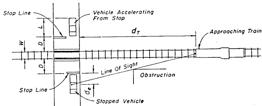
CASE B VEHICLE DEPARTING FROM STOPPED POSITION TO SAFELY CROSS RAILROAD TRACK
