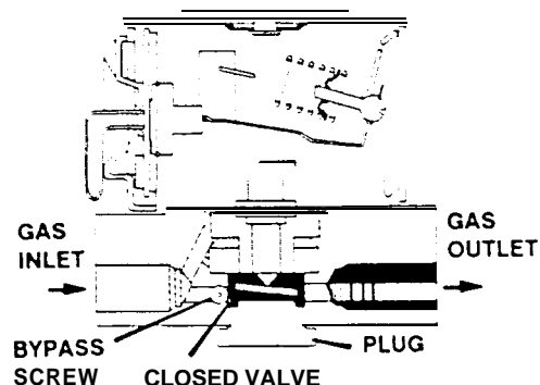
DIAL SHAFT
