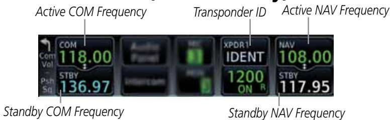
COM and NAV Radio Frequencies
