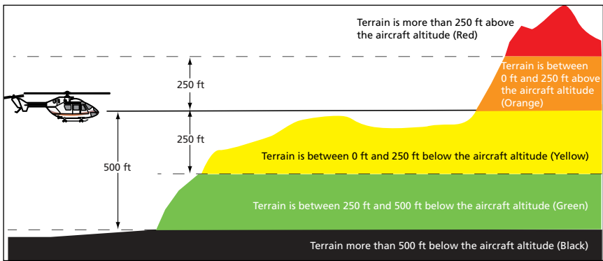
HTAWS Altitude/Color Correlation
